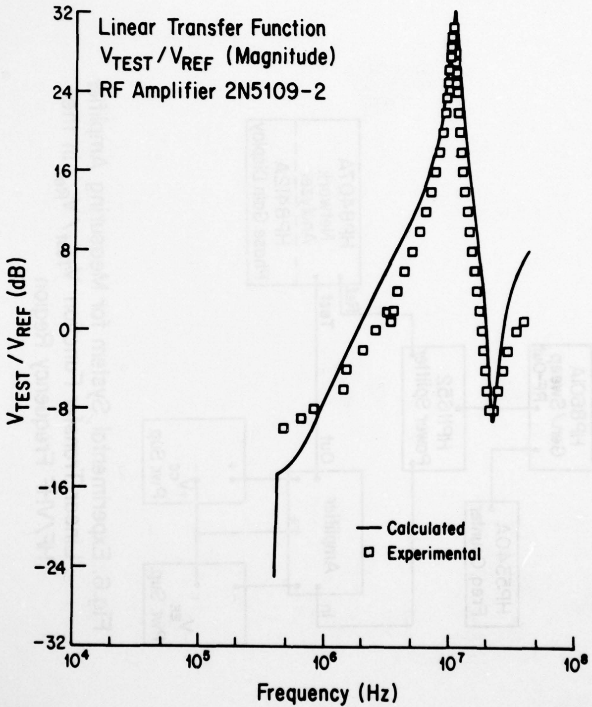
Fig. 7. Linear Transfer Function V_{TEST} / V_{REF} (Mag.)
