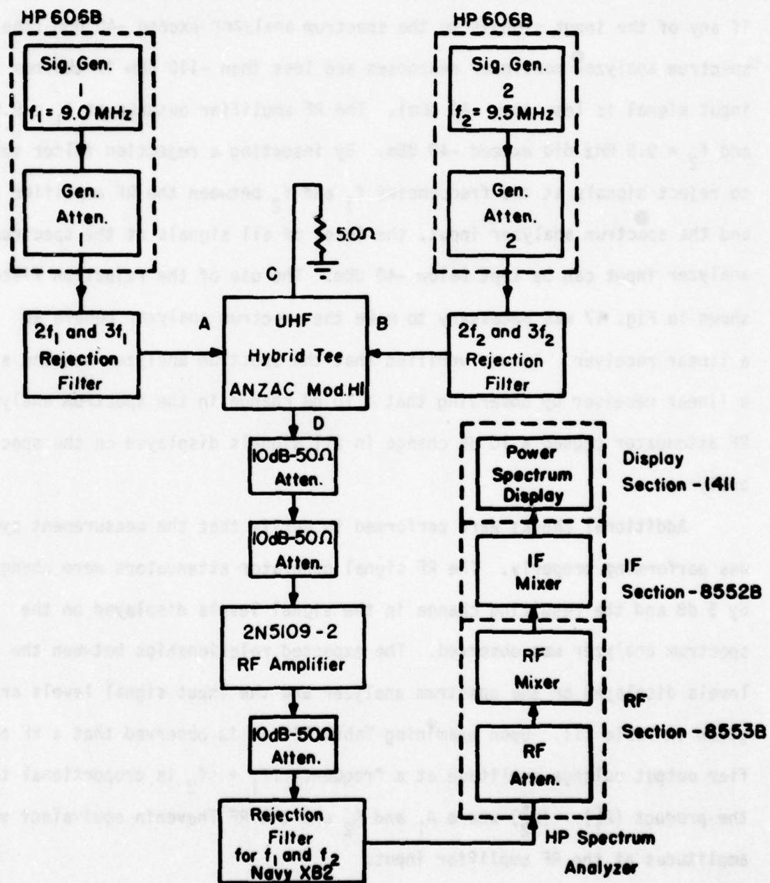
Fig. 17. Experimental System for Measuring H_3(f_2, f_2, -f_1)
