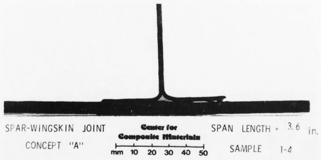
Figure 55: Specimen 1-4; Failed (Concept A; 3.6 inch span)
