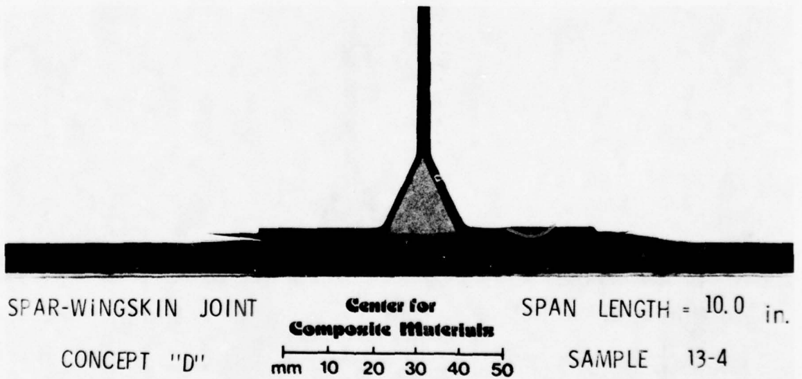
Figure 91: Specimen 13-4; Failed (Concept D; 10.0 inch span)
