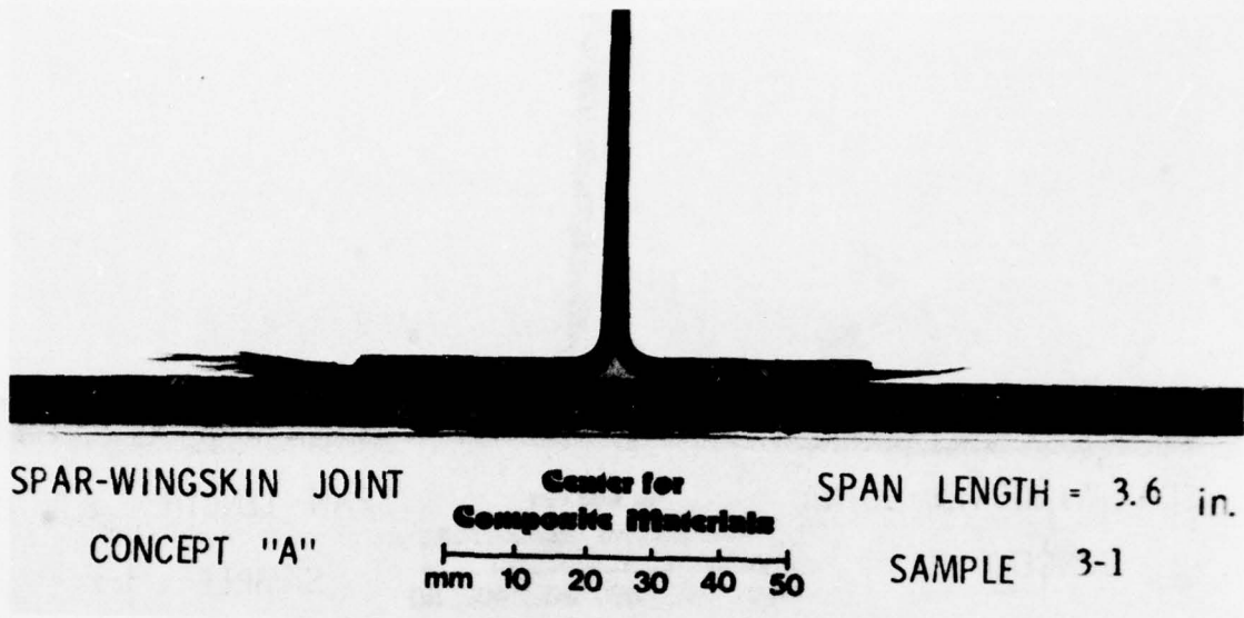
Figure 60: Specimen 3-1; Failed (Concept A; 10.0 inch span)
