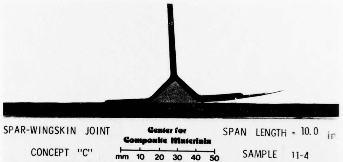
Figure 83: Specimen 11-4; Failed (Concept C; 10.0 inch span)
