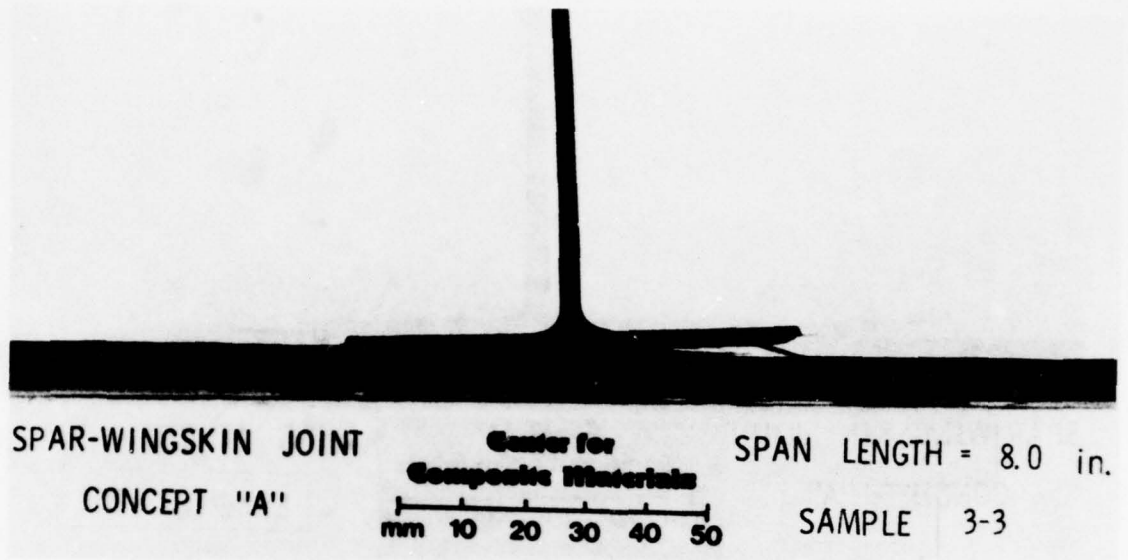
Figure 62: Specimen 3-3; Failed (Concept A; 6.0 inch span)
