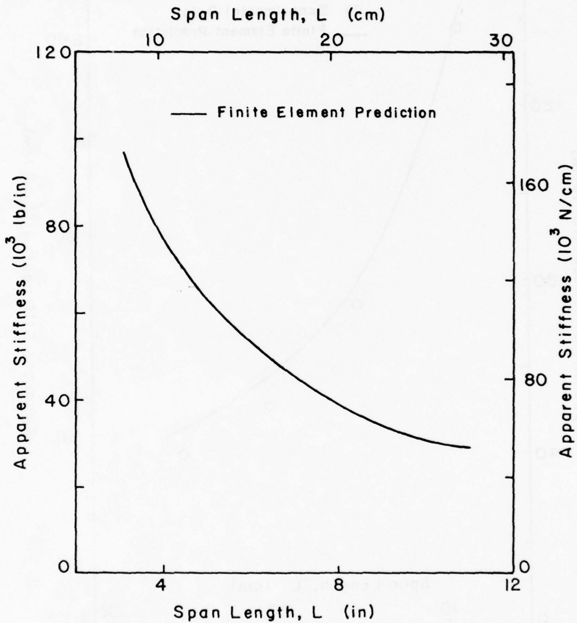
Figure 33: Influence of Span on Modulus for Concept "E"
