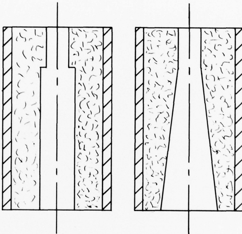
SHAPE 1 CYLINDRICAL
