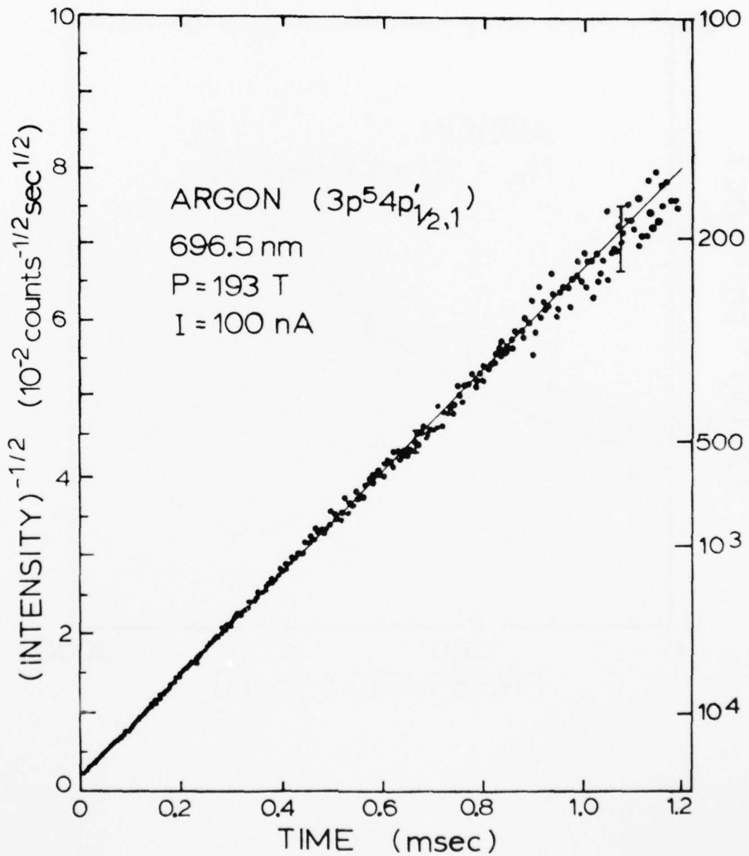
Figure 1. Inverse square root of the intensity of the argon ( 3p^5, 4p'_{1/2,1} + 3p^5, 4s_{1/2,2} ) transition plotted as a function of time.
