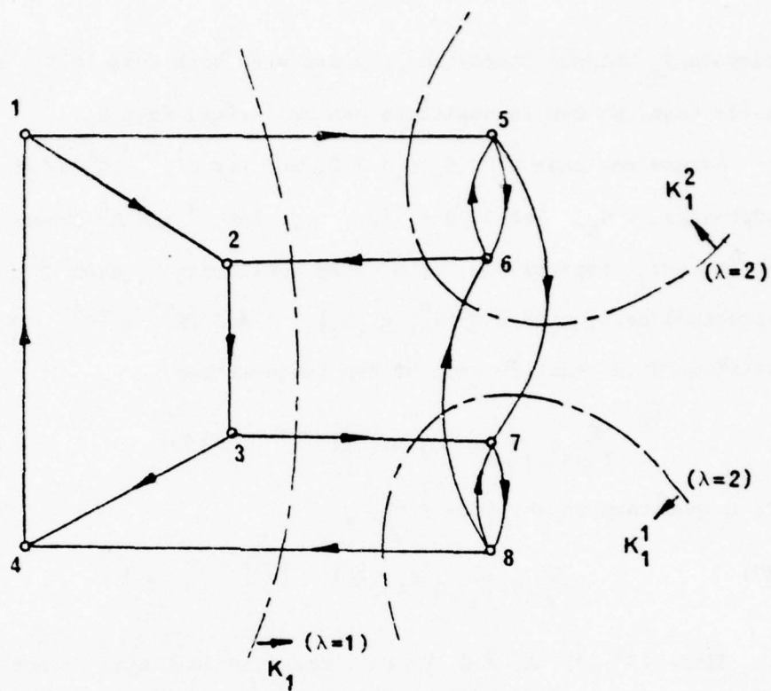
Fig. 7. G_0 after bounding procedure 4.
