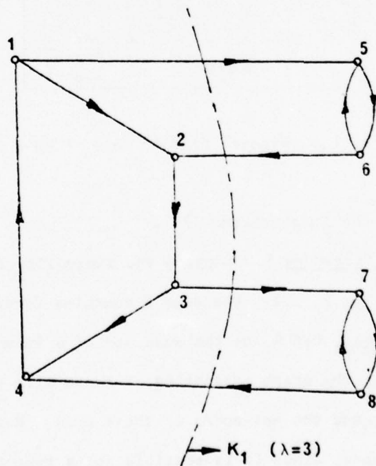
Fig. 5. Graph G_0 defined by the AP solution.
