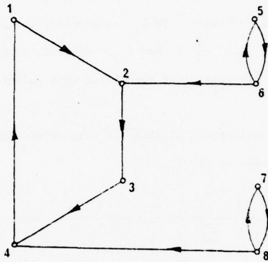
Fig. 5. Graph G_0 defined by the AP solution.
