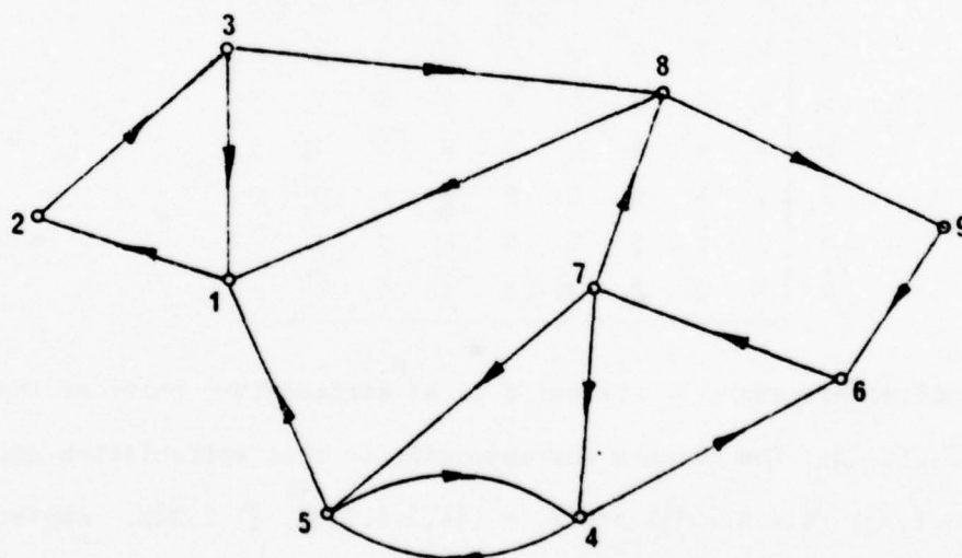
Fig. 4. G_0 after bounding procedure 3.
