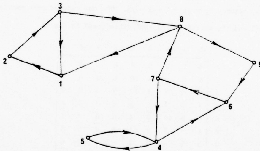
Fig 2. G_0 after bounding procedure 1.
