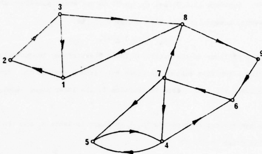
Fig. 3. G_0 after bounding procedure 2.
