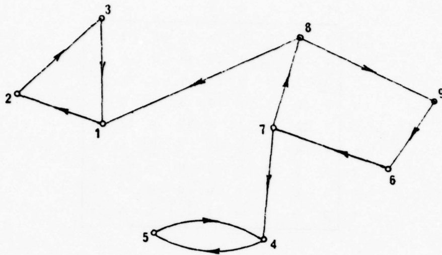
Fig 1. Graph G_0 defined by the AP solution.
