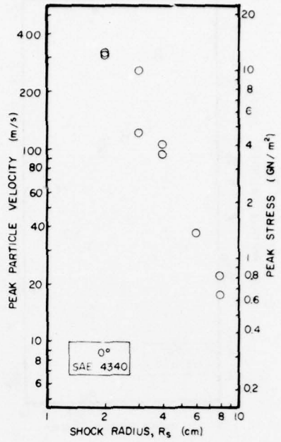
Figure 32. Peak Particle Velocity Versus Radius for SAE-4340 Steel at 0°
