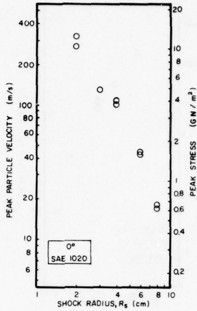
Figure 15. Peak Particle Velocity Versus Radius for SAE-1020 Steel at 0^\circ . ( 1 \text{ GN/m}^2 = 10 \text{ kbar} )
