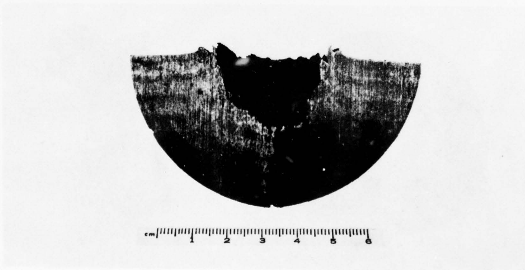
Figure 27. Post-impact Cross-section of a 8 cm Diameter Target
