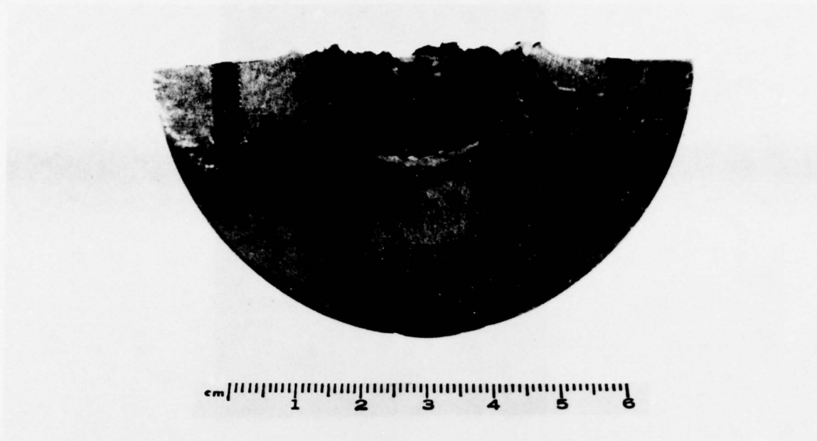
Figure 43. Post-impact Cross-section of an 8 cm Diameter 4340 Target
