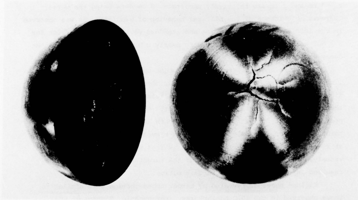
Figure 42. Post-impact Condition of an 8 cm Diameter 4340 Target
