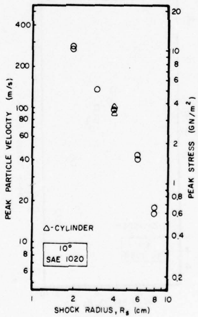
Figure 16. Peak Particle Velocity Versus Radius for SAE-1020 Steel at 10^\circ
