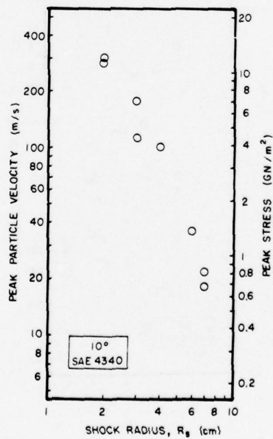
Figure 33. Peak Particle Velocity Versus Radius for SAE-4340 Steel at 10°
