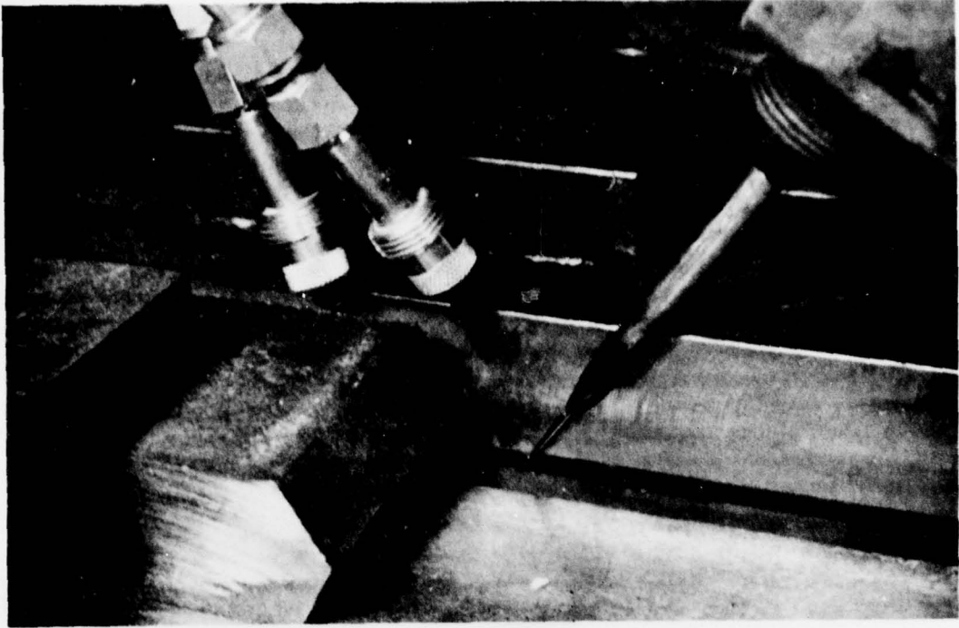
Figure 10 Arrangement of Wire
