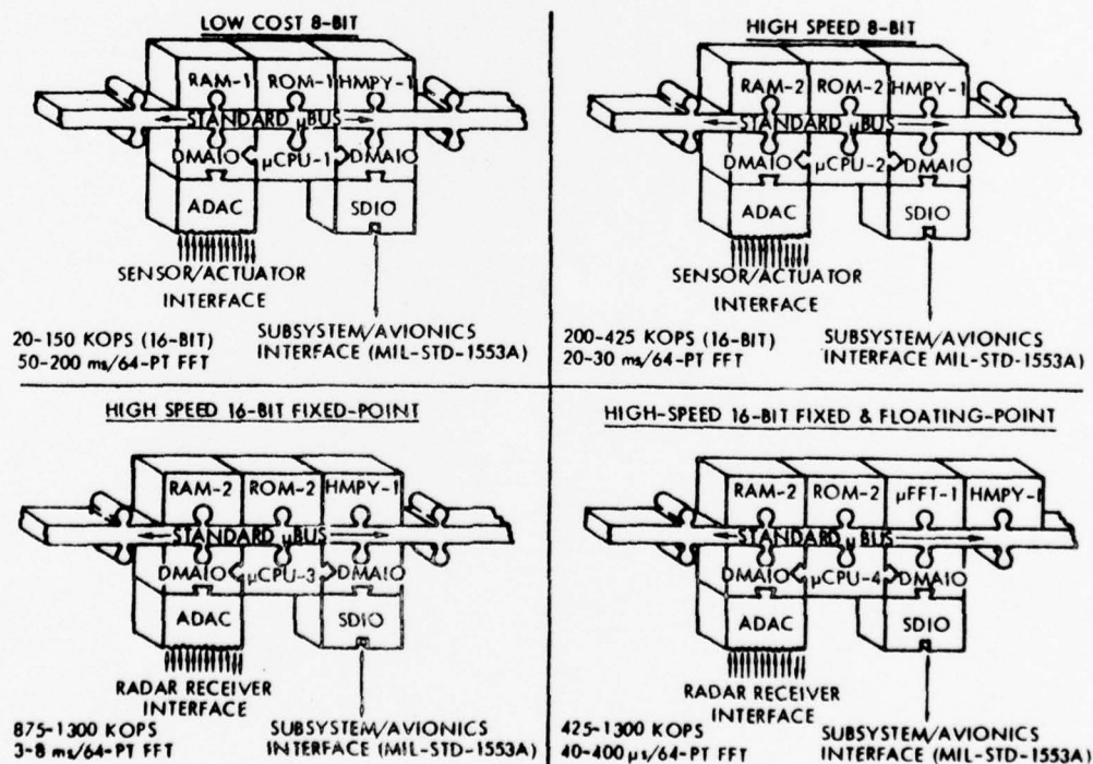
Figure 2 - Macromodular Microcomputer Family
