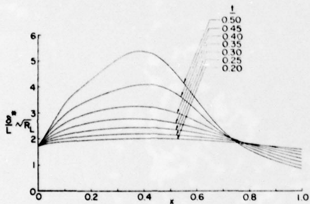
Fig. 4 Variation of dimensionless displacement thickness \delta^* / L \sqrt{R_L} with x for various values of t .
