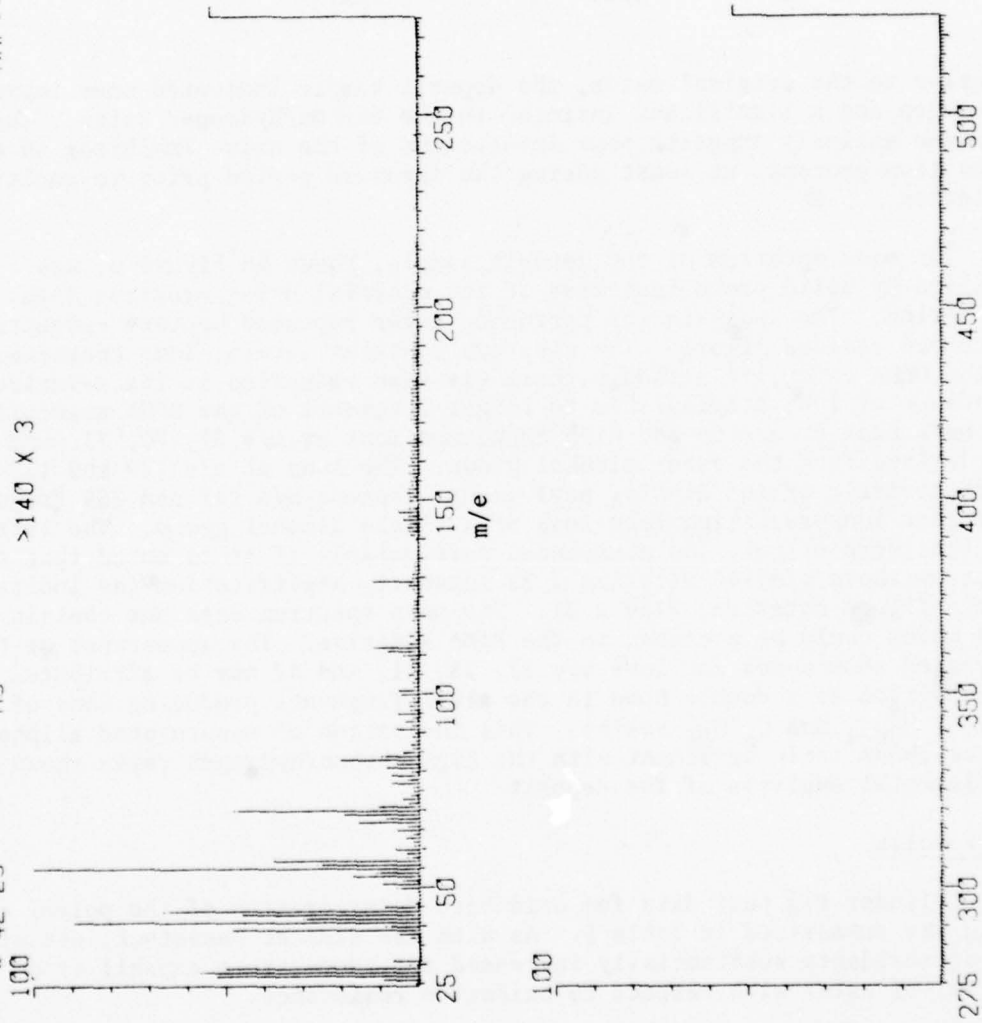
FIGURE 6. MASS SPECTRUM FOR TEST NO. 67 DEPOSIT SAMPLE
