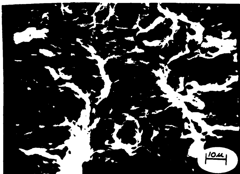
Figure 24: Fracture surface. Notched .025 in. specimen (air #111). Completed 1.51 \times 10^7 cycles at \sigma_i = 12,968 psi in air followed by 2.6 \times 10^3 cycles at \sigma_i = 36,655 psi in air. Transition from stage 2 crack propagation to ductile/fast fracture. Total crack propagation in 1.51 \times 10^7 cycles \approx .0026 in. 1000X.
