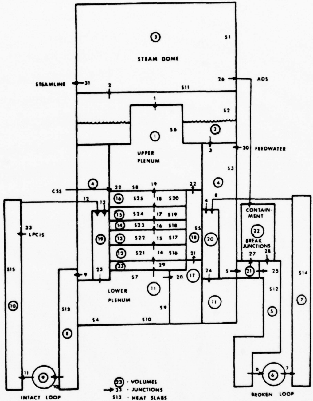
FIGURE 1 RELAP4 MODEL OF G. E. BWR
