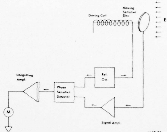
Figure 56 Field Meter
