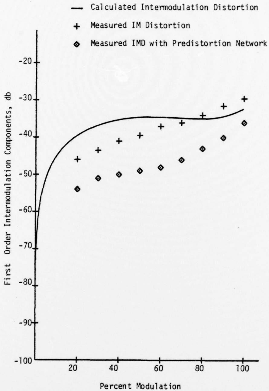
Figure 5-19. Intermodulation Distortion vs Percent Modulation for TIL31 Diode #1.
