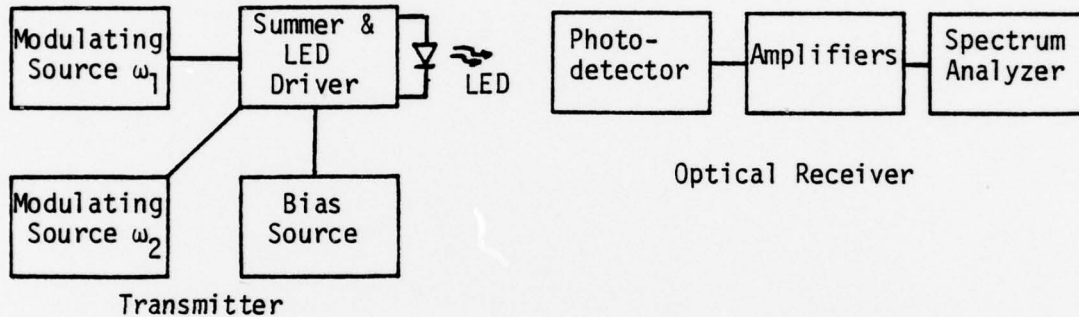
Figure 2-1. Block Diagram for Measuring LED Linearity.
