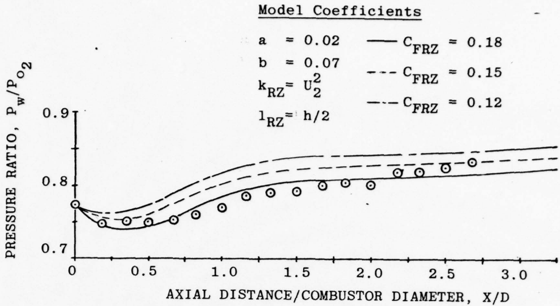
a) Effect of Recirculation Zone "Skin Friction" Coefficient on Wall Static Pressure Distribution
