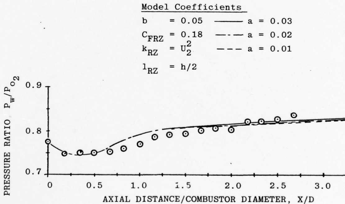
d) Effect of Shear Layer Growth Rate on Wall Static Pressure Distribution
