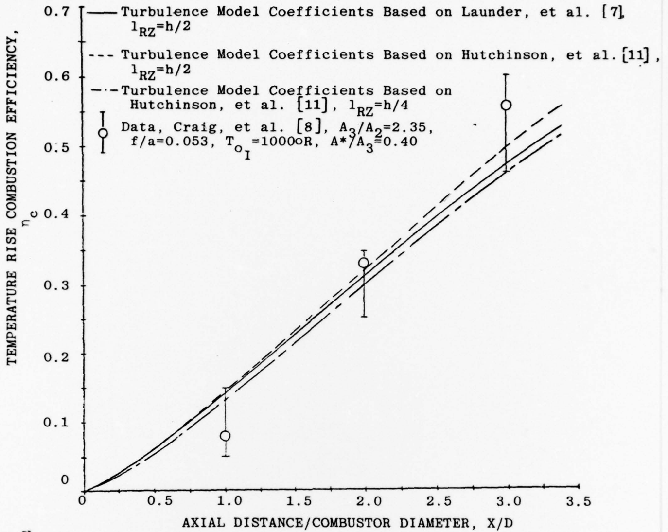
a) Combustion Efficiency
