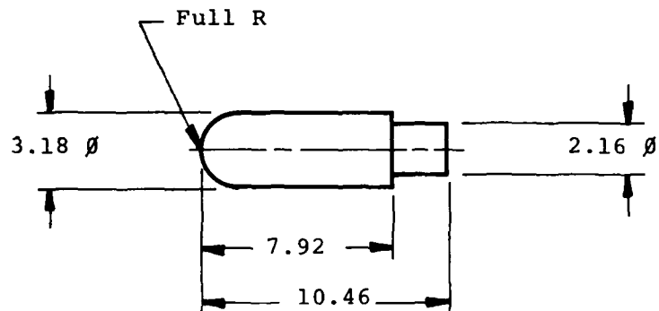
(A) Standard Hemispherical Cathode
