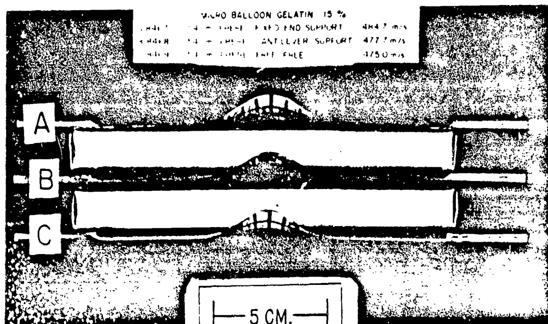
Figure 29. Effect of method of specimen mounting on damage.
