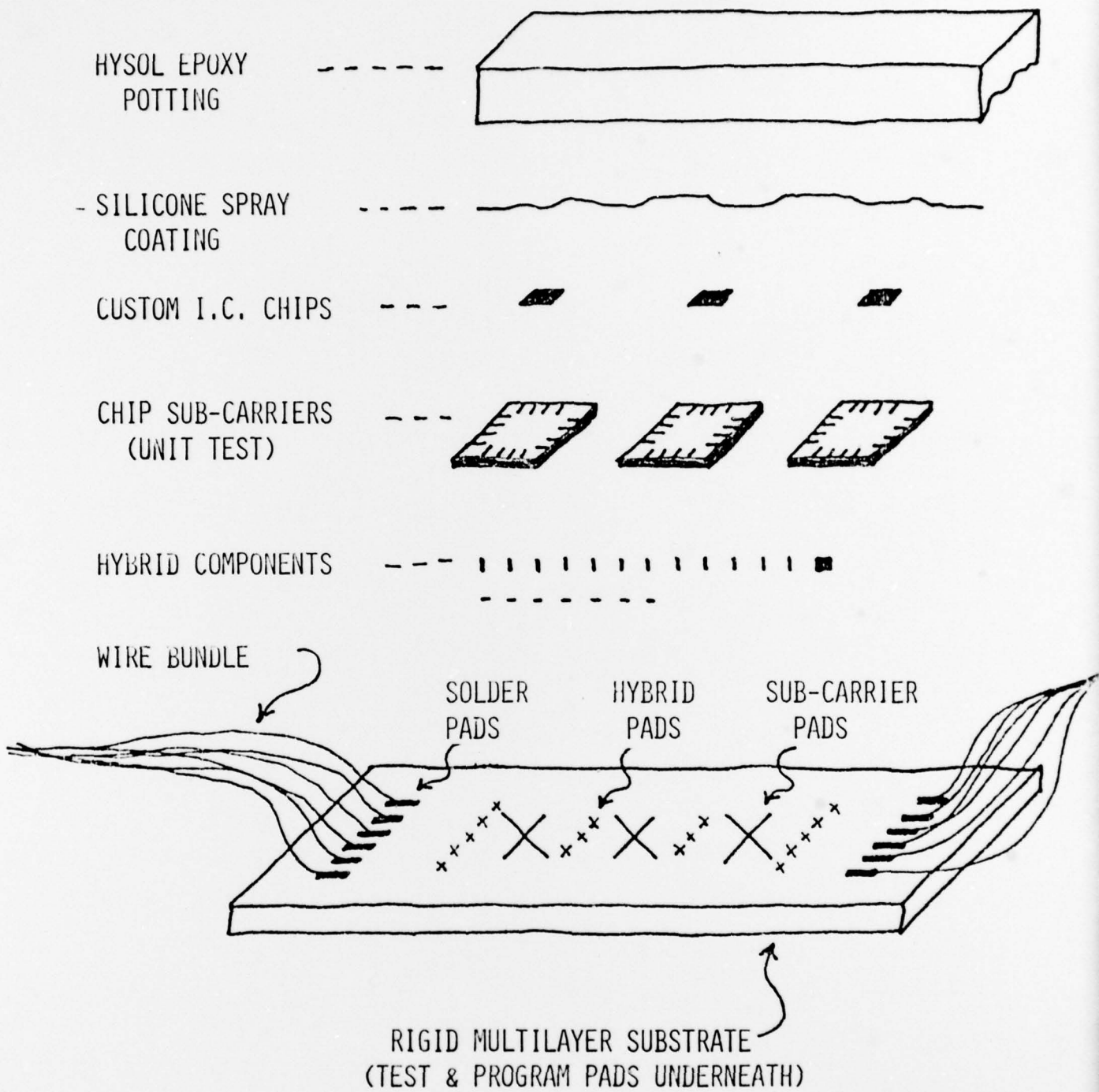
Figure 2-2. Telemetry Unit Packaging
