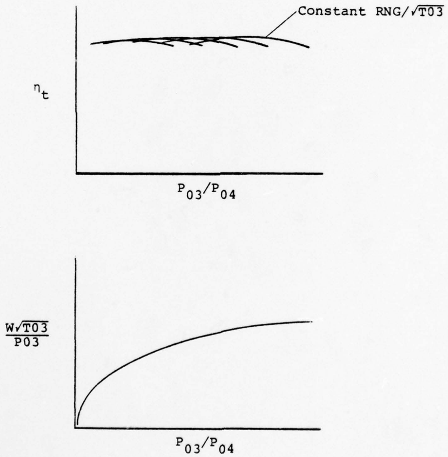
FIGURE 4-4: Single Line Turbine Characteristics [4]
