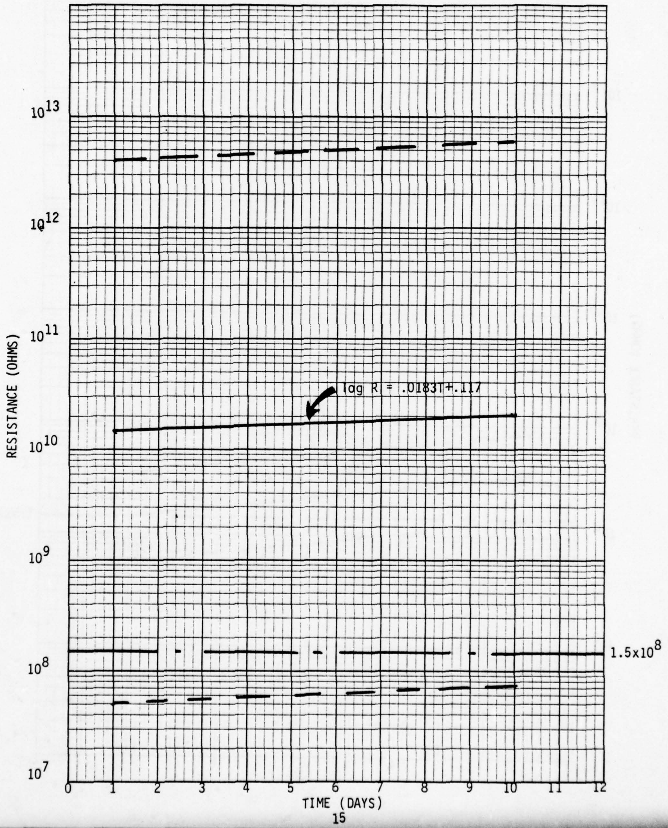
FIGURE 4. 72 HOUR DELAY (A, B, AND C FUSING FLUIDS) CONTROLS RESISTANCE VS TIME
