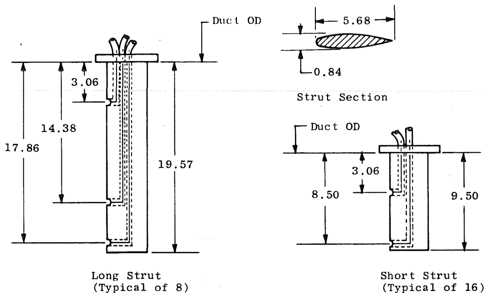
Strut Details
