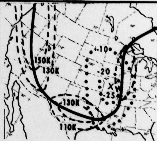
Figure 123d: Composite
