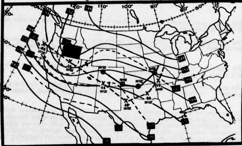
Figure 9: 18-20 Dec 1973
