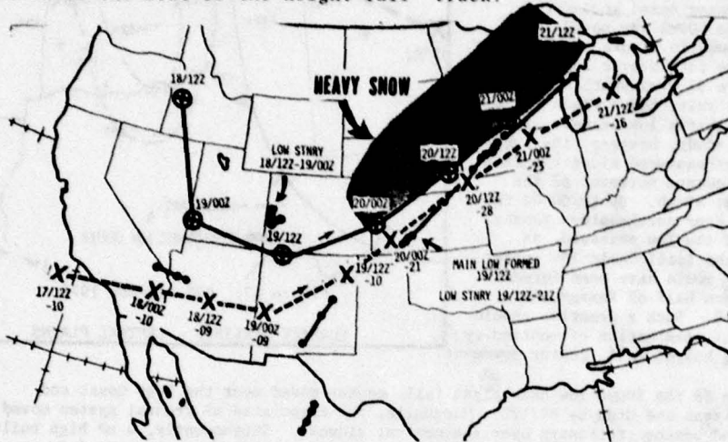
Figure 55: Composite, 18 - 21 Nov 1975
