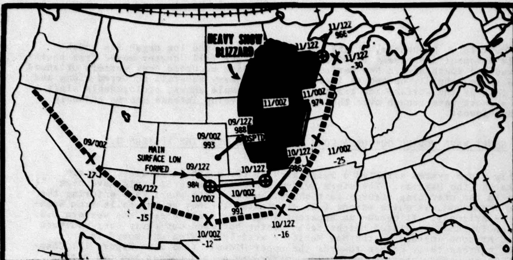
Figure 51: Composite, 8-11 Jan 1975
