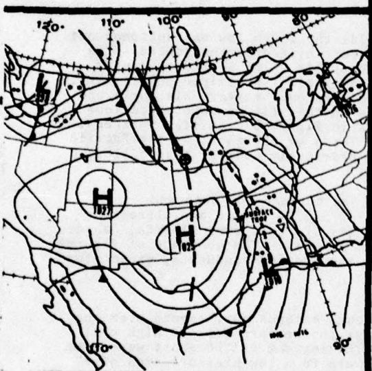
Figure 38c: 12Z 26 Nov 1975
