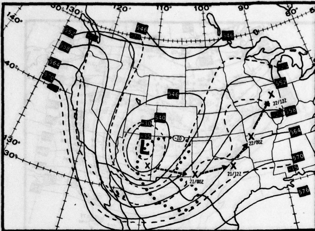
Figure 12c: 12Z 20 Jan 73
