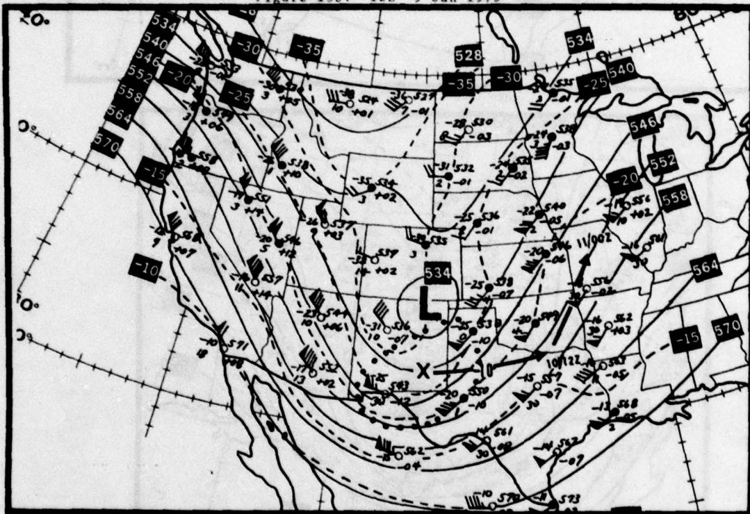
Figure 13c: 00Z 10 Jan 1975
