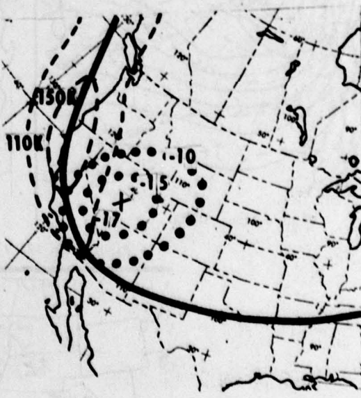
Figure 114d: Composite
