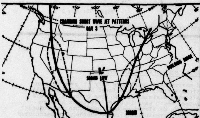
Figure 1c: Day 3
