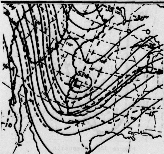
Figure 118c: 500mb
