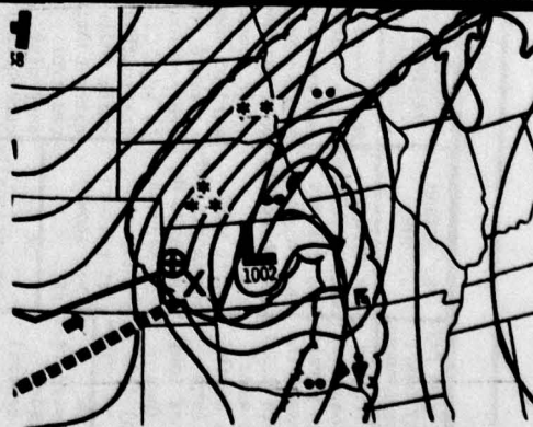
Figure 94: 00Z 20 Nov 1975
