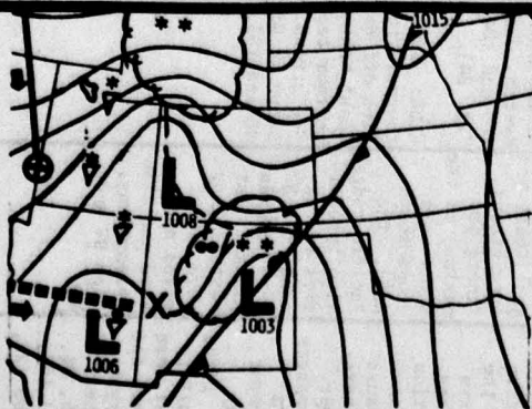
Figure 93: 00Z 19 Nov 1975
