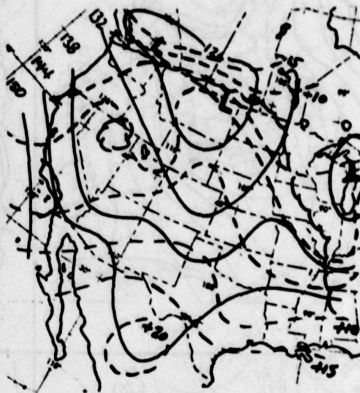
Figure 114b: 850mb
