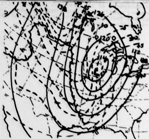
Figure 123b: 850mb
