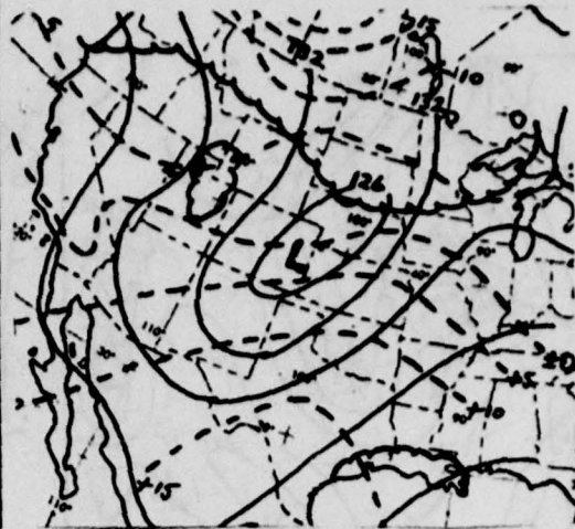
Figure 115b: 850mb
