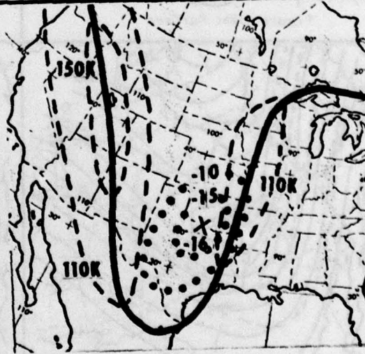
Figure 120d: Composite
