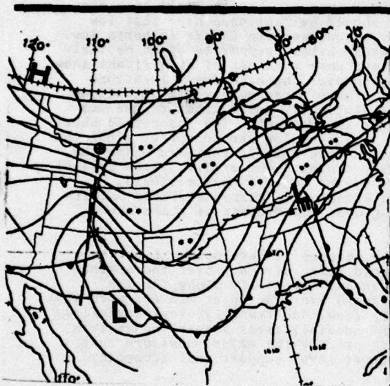
Figure 37c: 12Z 11 Jan 1963
