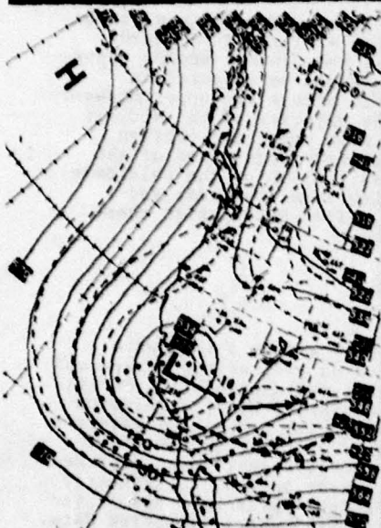
Figure 15c: 12Z 3 Mar 1976
