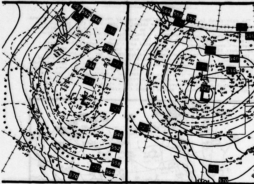
Figure 17c: 12Z 31 Dec 1975
