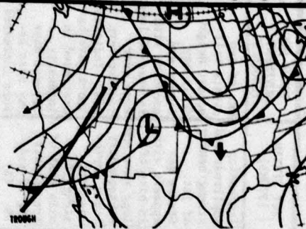
Figure 90: Prevailing High
