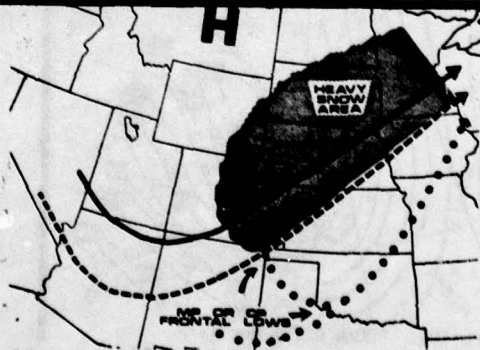
Figure 109: Prevailing High
