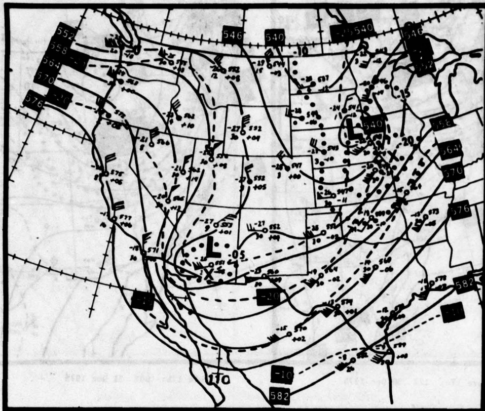
Figure 16c: 00Z 3 Jan 1975
