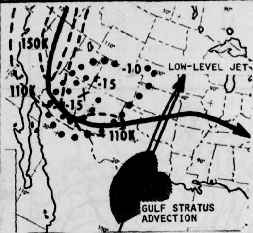
Figure 115d: Composite
