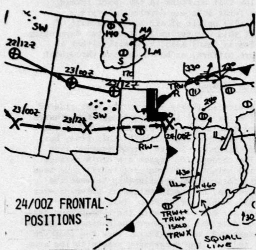
Figure 70c: 2335Z 23 Dec 73
