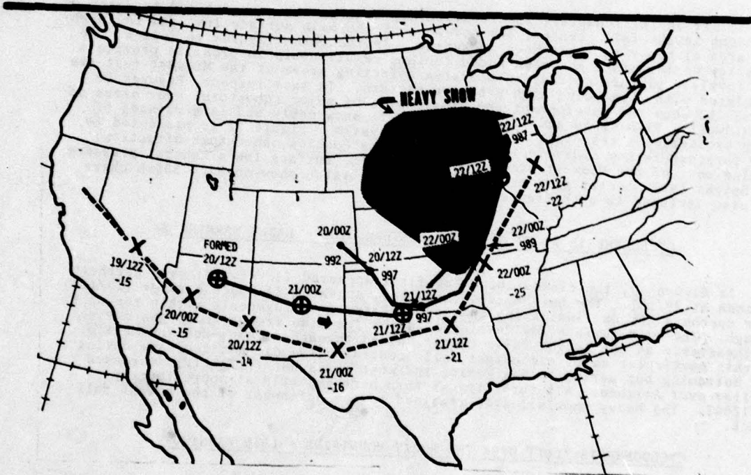
Figure 50: Composite, 19-22 Jan 1973
