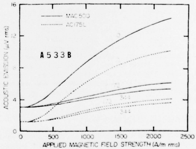
Fig. 2 Acoustic emission vs. applied magnetic field strength for five materials at 175 kHz without applied stress.
