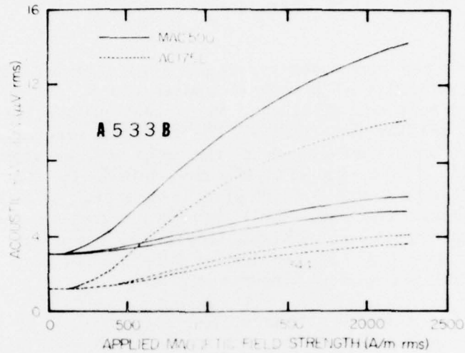
Fig. 3 Acoustic emission vs. applied magnetic field strength for A533B steel at three stress levels, 0, 172 and 344 MPa. Solid lines for 500 kHz and dotted lines for 175 kHz.
