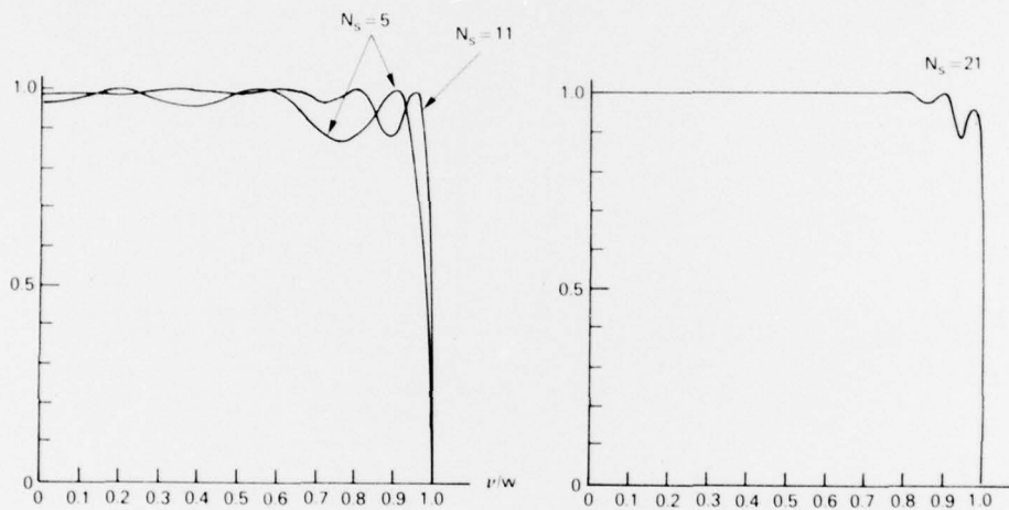
Fig. 1 - Q_b^2/Q_c^2 vs \nu/W
