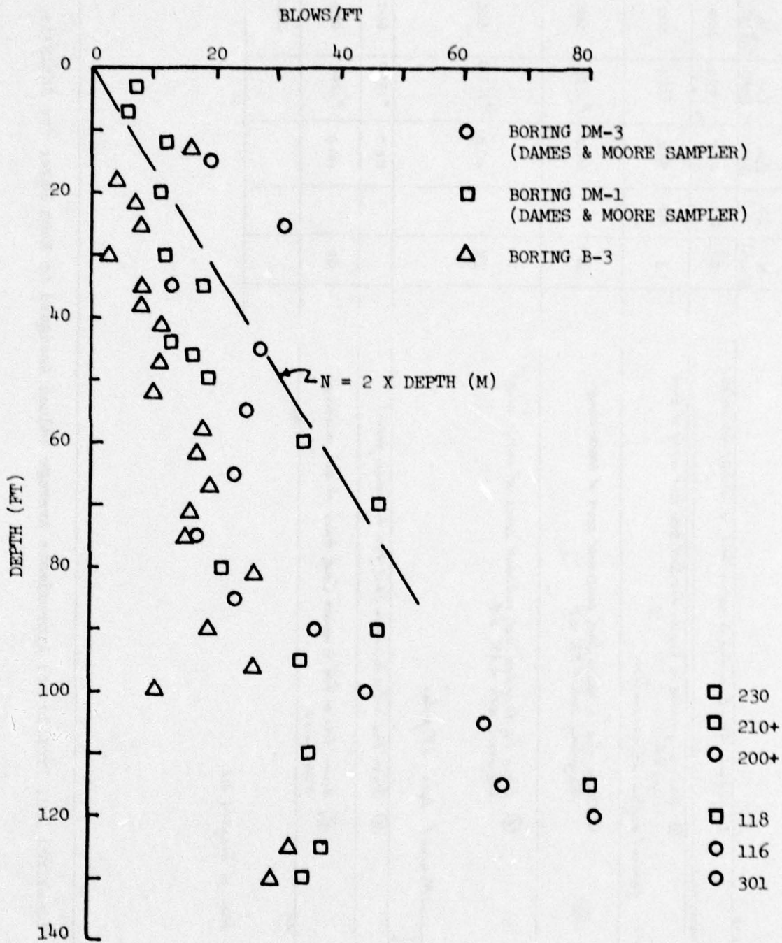
Figure 2. Blow Counts Presented as a Function of Depth
