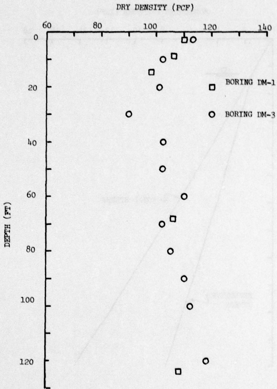
Figure 3. Dry Density as a Function of Depth
