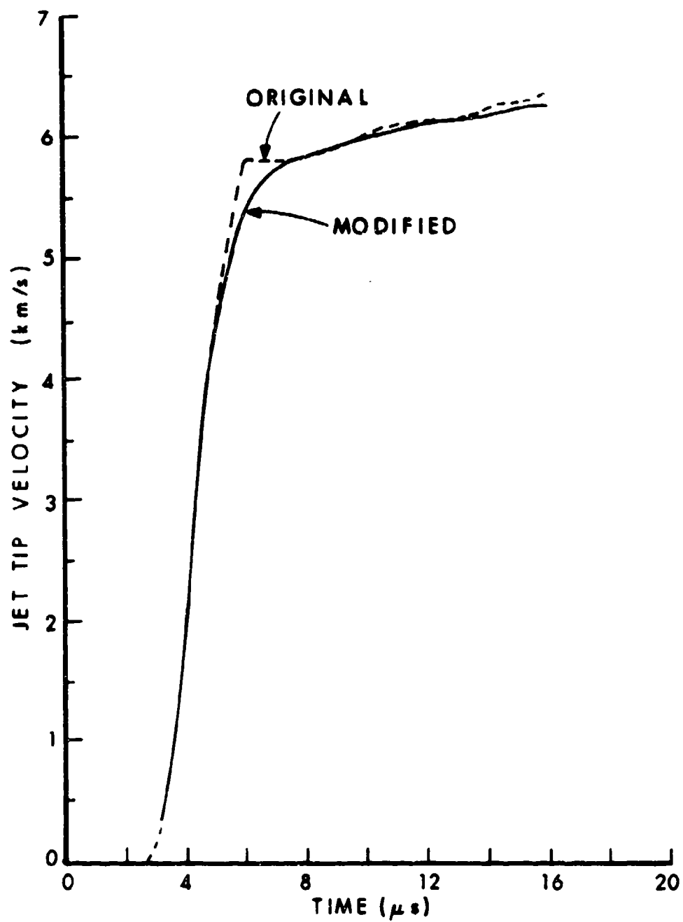
Figure 14. Comparison of the Jet Tip Velocity-Time Histories
