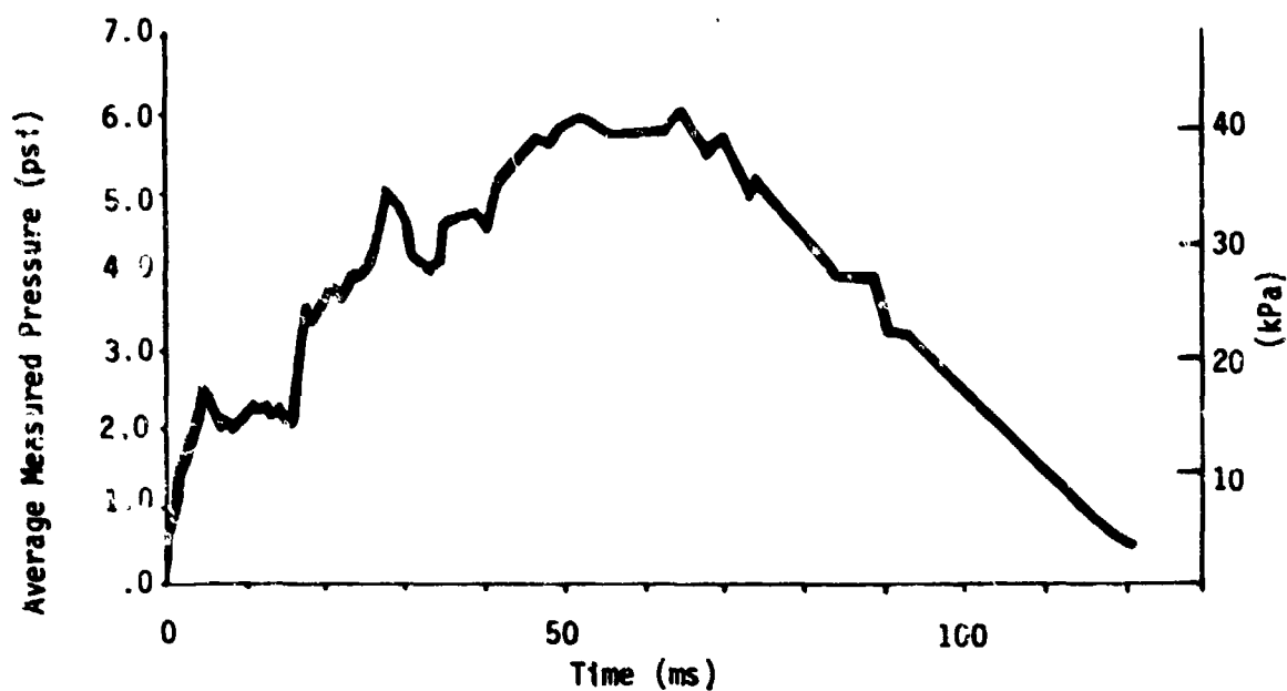
Fig. 27. Average Pressure at a Gauge in the Side Wall of a Room with a "20%" Window. (See also Fig. 21.)
