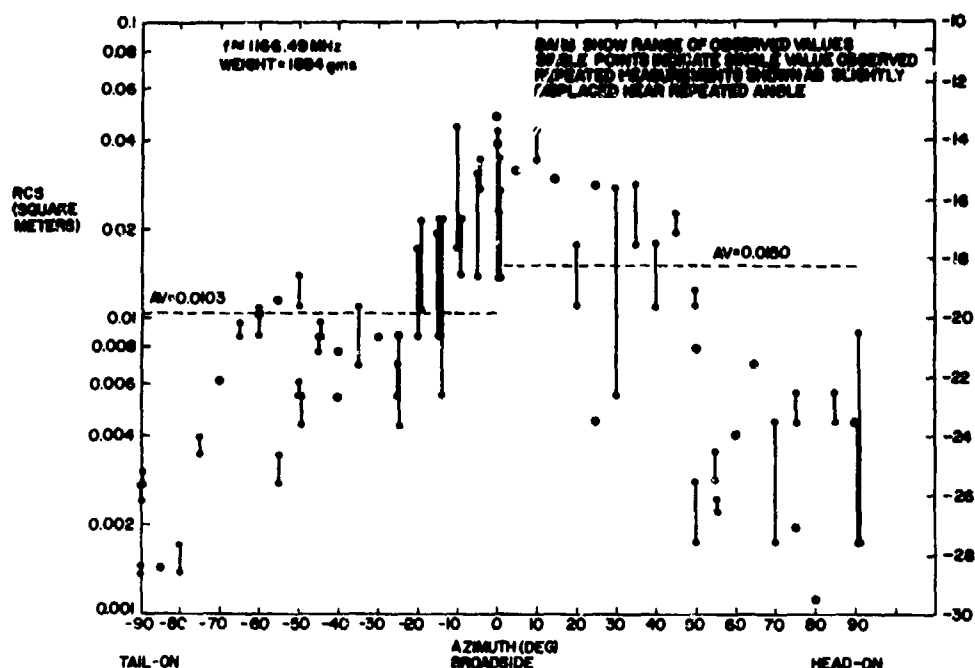
Figure 7. Measured Radar Cross Section—Duck No. 1, Horizontal Polarization
