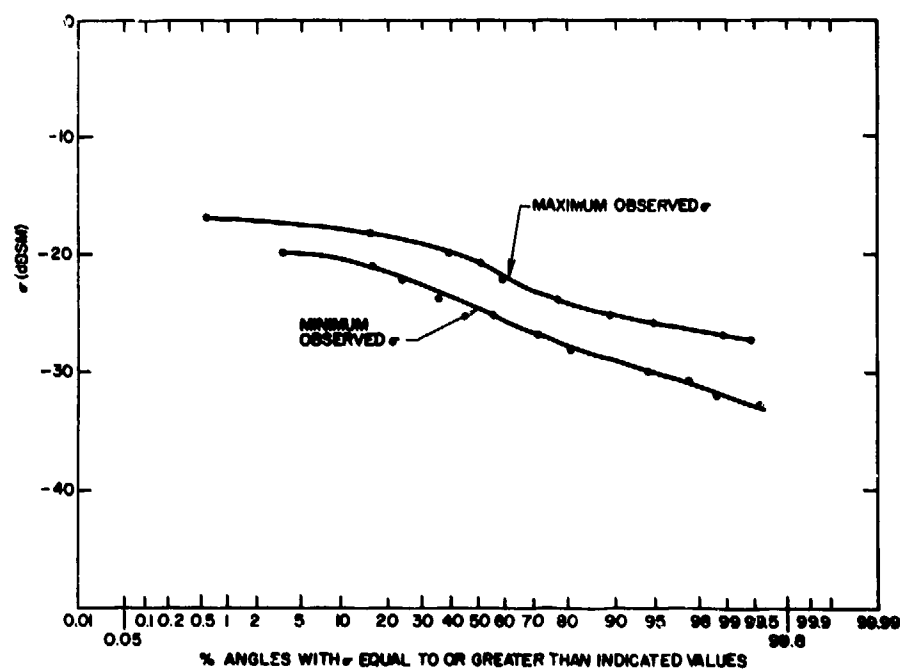
b. Vertical Polarization, Ducks
