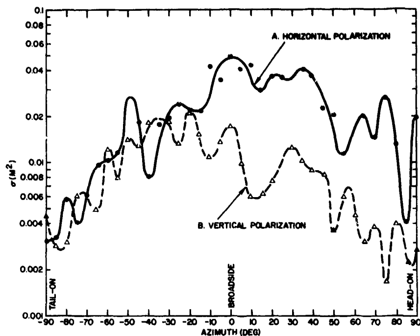
Figure 15. Smooth Curve Fit to Maximum RCS of Ducks, (a) Horizontal Polarization, (b) Vertical Polarization
