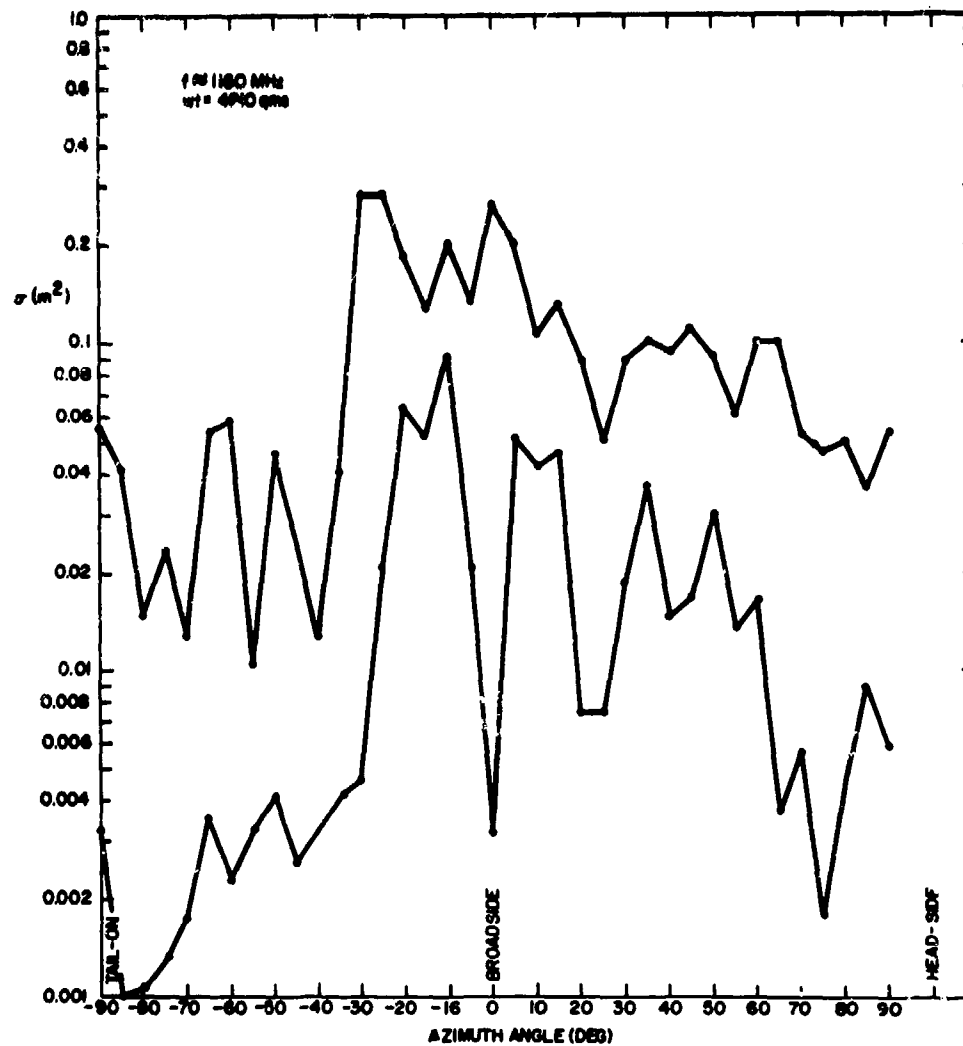
Figure 14. Maximum and Minimum Measured RCS of Birds (Cont.)
