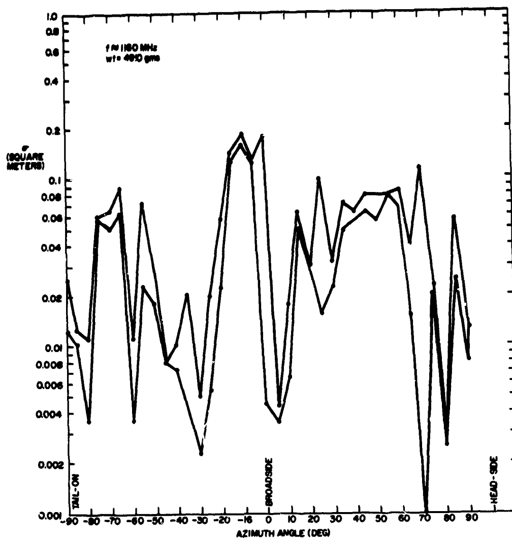
d. Goose, Vertical Polarization
