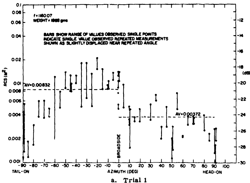
Figure 9. Measured Radar Cross Section - Duck No. 2, Vertical Polarization
