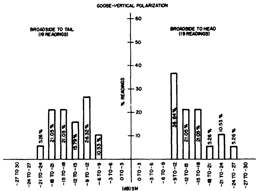
d. Goose Vertical Polarization
