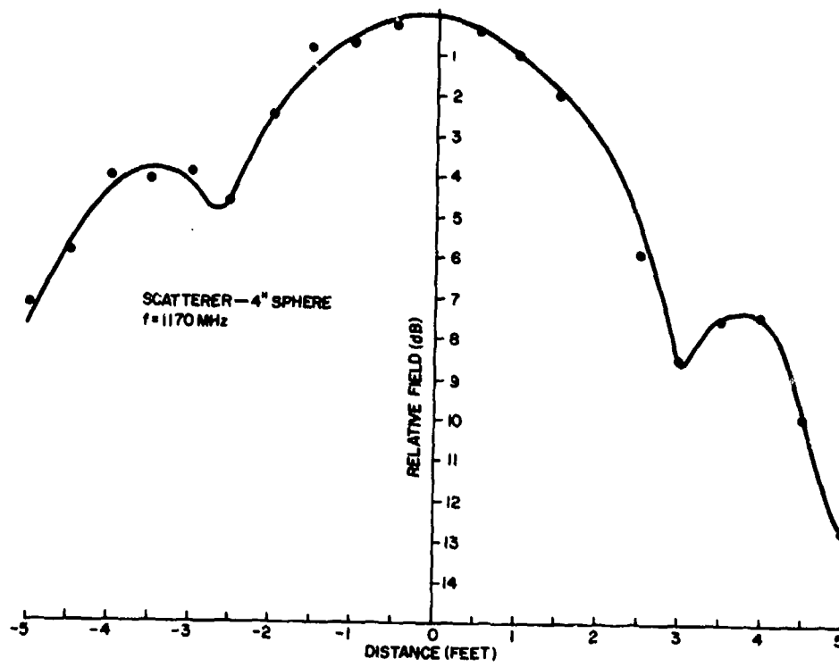
Figure 5. Horizontal E-Field (Horizontal Polarization)
