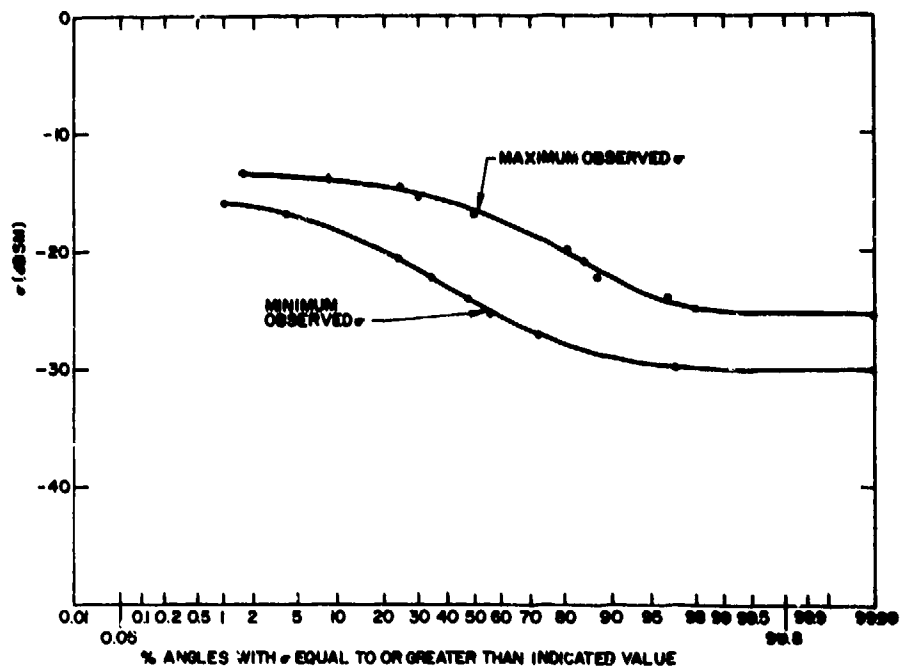
a. Horizontal Polarization, Ducks
