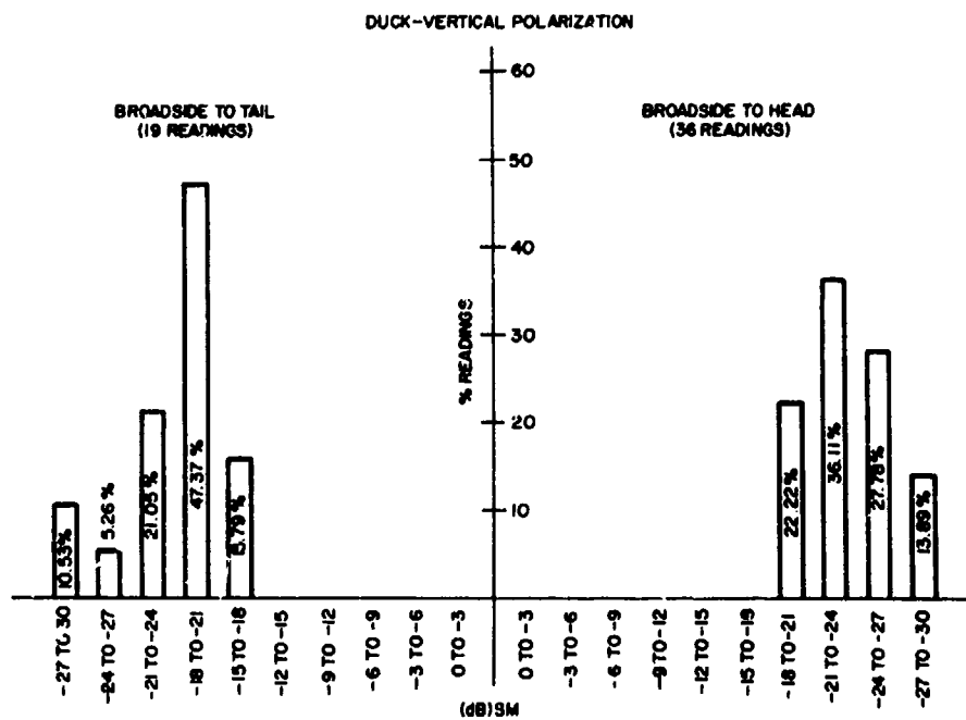
b. Duck Vertical Polarization
