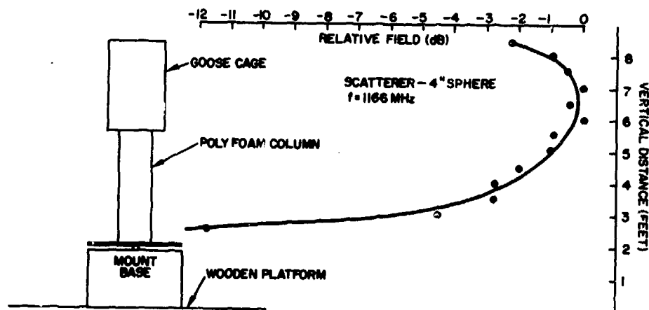
Figure 6. Vertical E-Field (Vertical Polarization)
