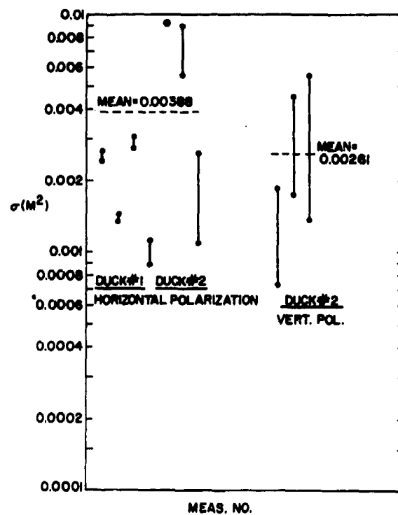
Figure 13. Comparison of Repeated Duck Measurements (Cont.)
