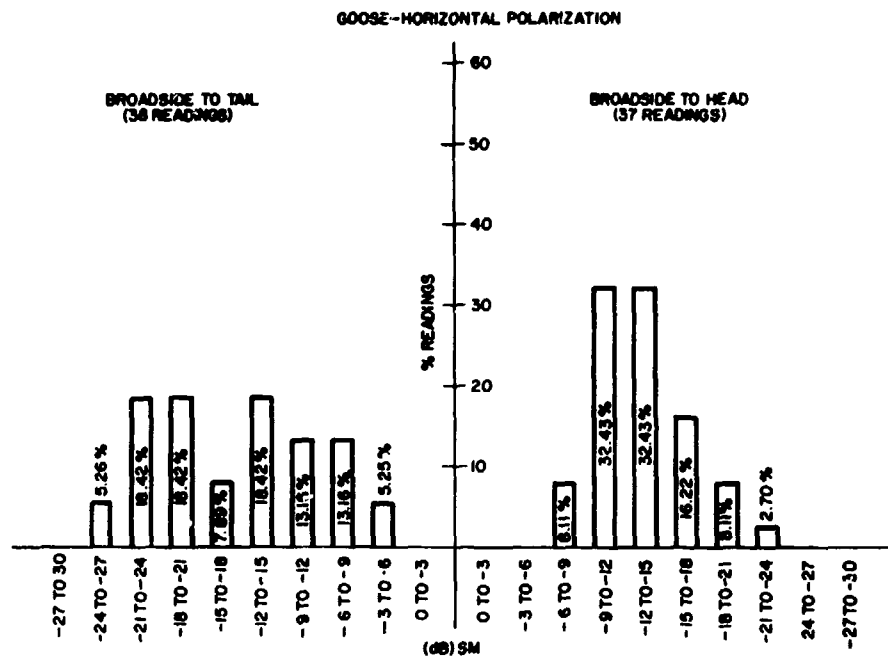
c. Goose Horizontal Polarization
