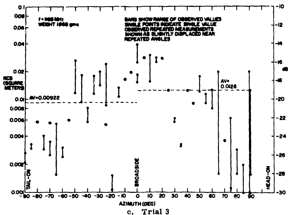
Figure 8. Measured Radar Cross Section - Duck No. 2, Horizontal Polarization (Cont.)
