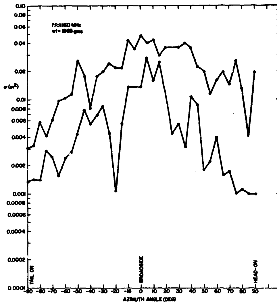
a. Duck, Horizontal Polarization
