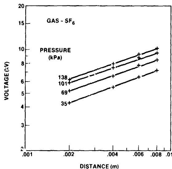
Fig. 6 — Flashover voltage of \text{SF}_6
