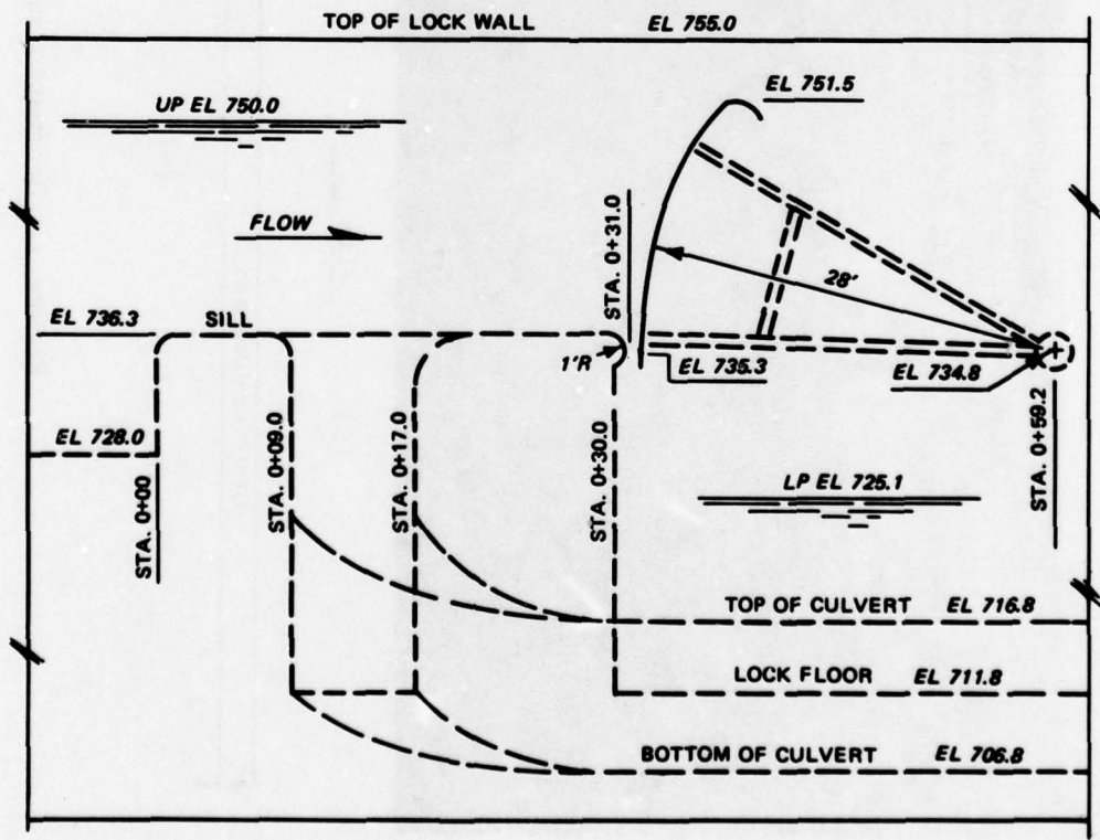
b. Cross section, upstream to downstream, Lower Lock Figure 4. Details of existing intakes
