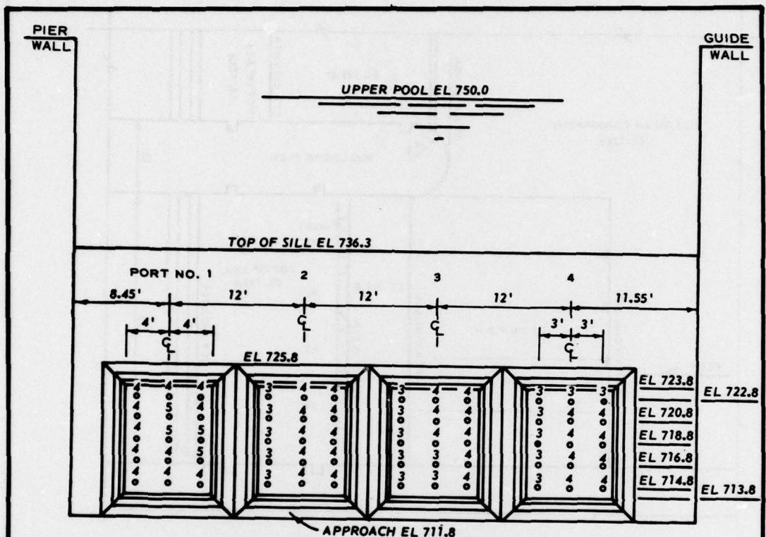
VELOCITIES AT INTAKE PORT FACE
