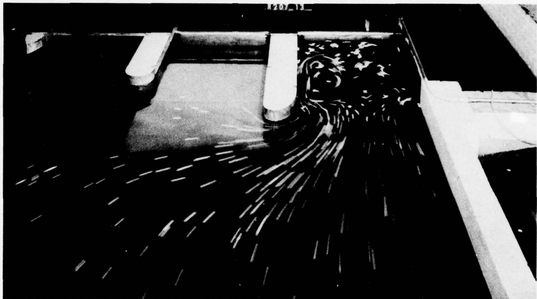
Photo 4. Surface currents during steady-flow peak discharge conditions, type 3 design, time exposure 5 sec; upper pool el 750.0, lock chamber el 732.0, culvert valve fully open
