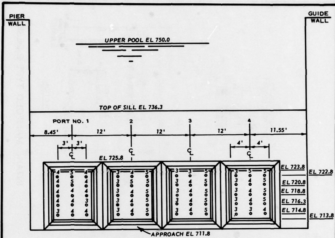
VELOCITIES AT INTAKE PORT FACE
