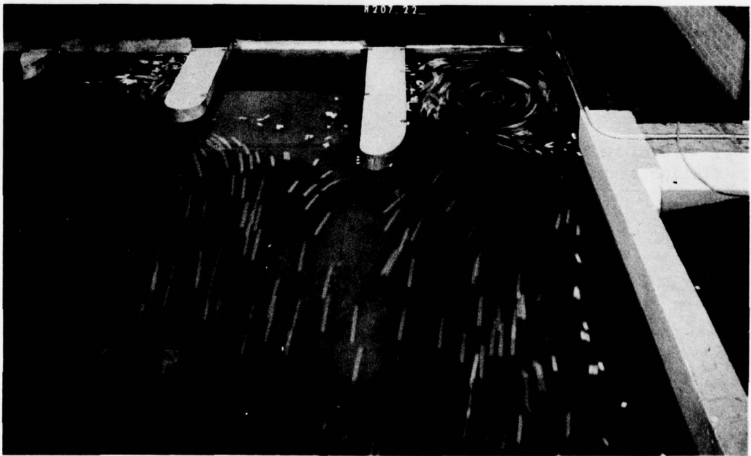
Photo 5. Surface currents during steady-flow peak discharge conditions through intake, type 3 design, culvert valve fully open; upper pool el 750.0, lock chamber el 732.0, auxiliary lock gate closed. Dam gates 1 and 2 open 3 ft, each gate passing 4,920-cfs discharge; dam gate 3 open 3.2 ft, passing 5,230-cfs discharge. Tailgate downstream of dam el 727.0; total discharge through dam approximately 15,070 cfs
