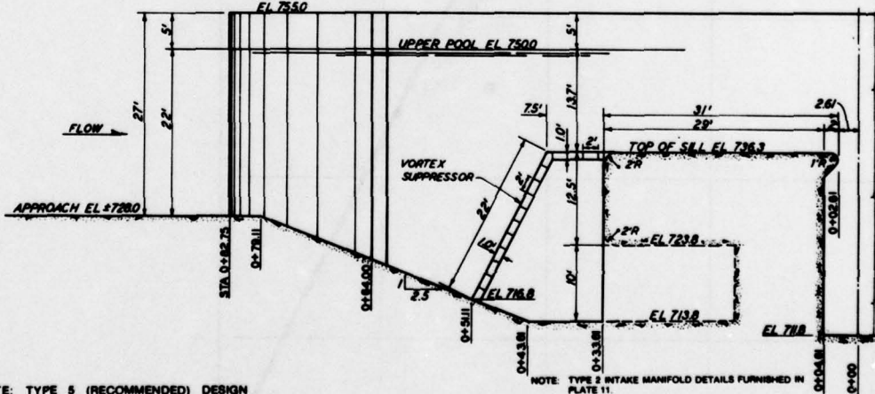
SECTION ALONG LOCK APPROACH LOOKING LEFT
