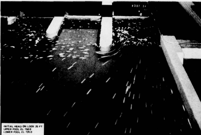
Photo 13. Surface currents during filling operation, type 5 (recommended) design, time exposure 5 sec; river discharge 0 cfs, discharge exceeded 100 percent of time, 4.14-min valve time (sheet 1 of 2)
