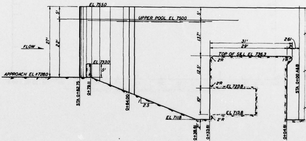
SECTION ALONG LOCK APPROACH LOOKING LEFT
