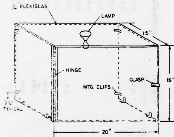
SCRATCH GAUGE ENCLOSURE FIGURE A-3
