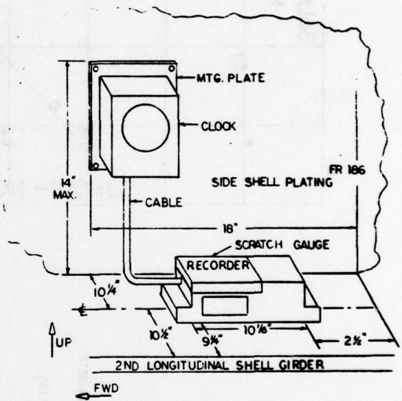
COMPONENT LAYOUT FIGURE A-2
