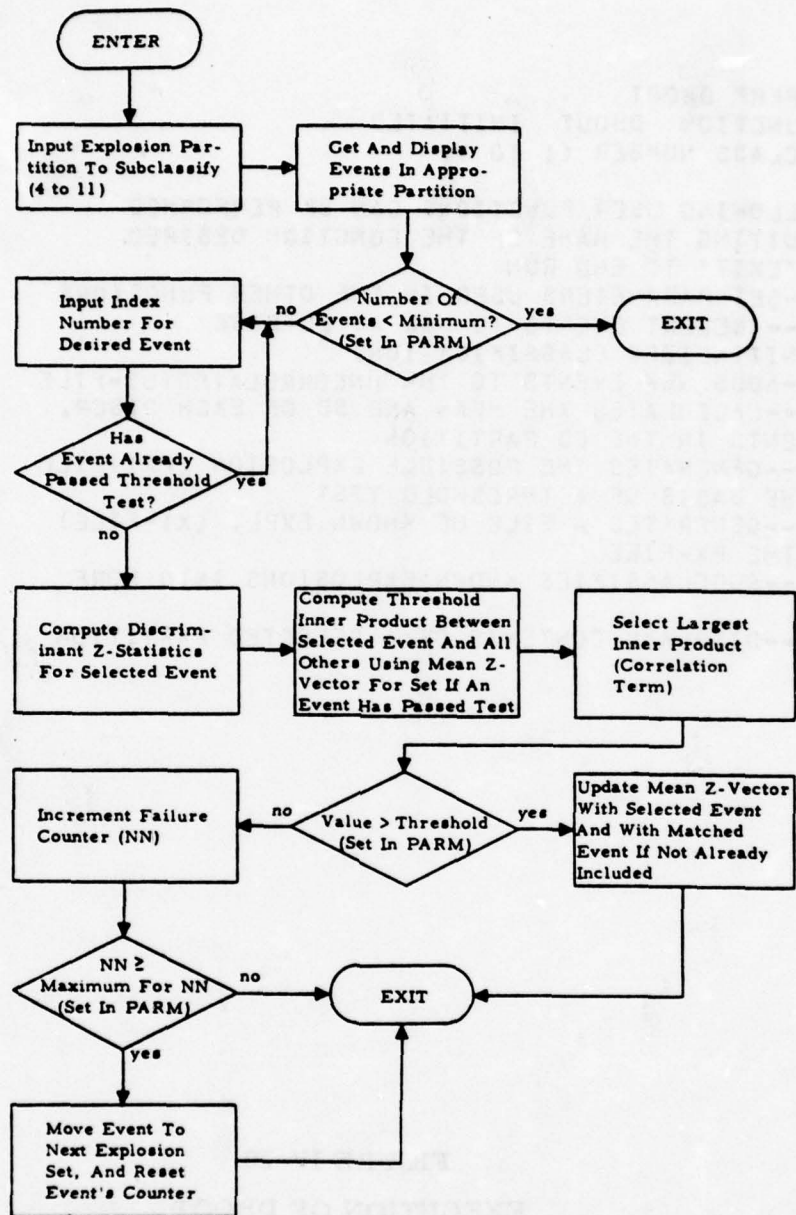
FIGURE IV-19 USER FUNCTION SUBEX
