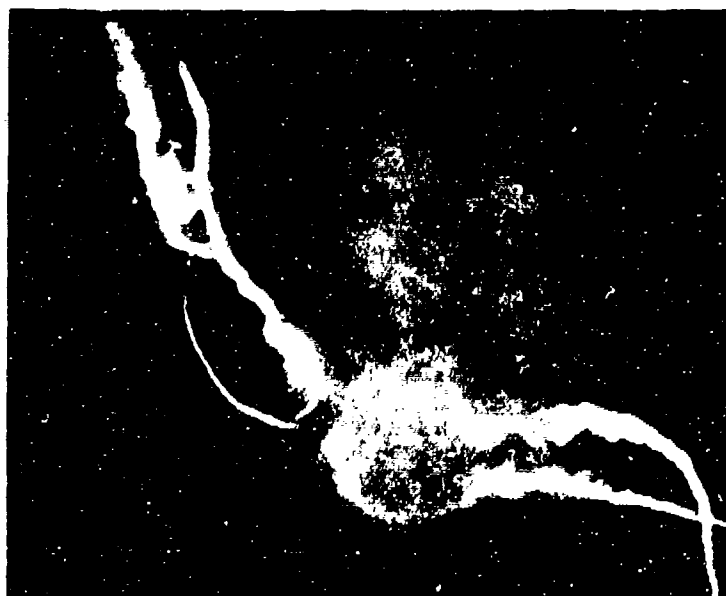
Figure 7. Vortex Bursting Behind a Cessna 170 (Ref. 15)
