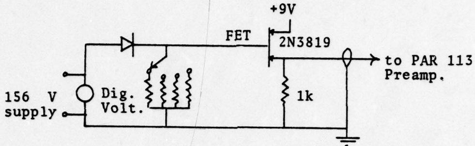
FIG. (15) Circuit for Avalanche Detectors
