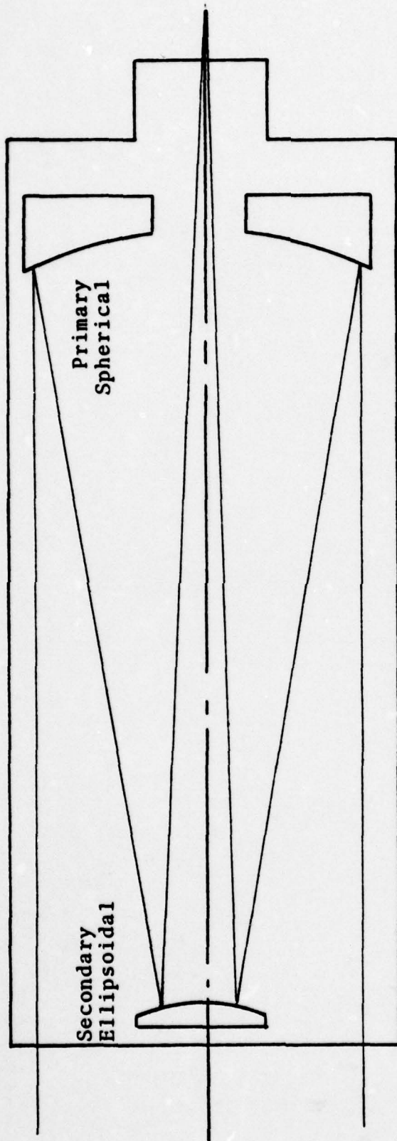
FIG. (3) Dah1-Kirkham Astronomical Telescope
