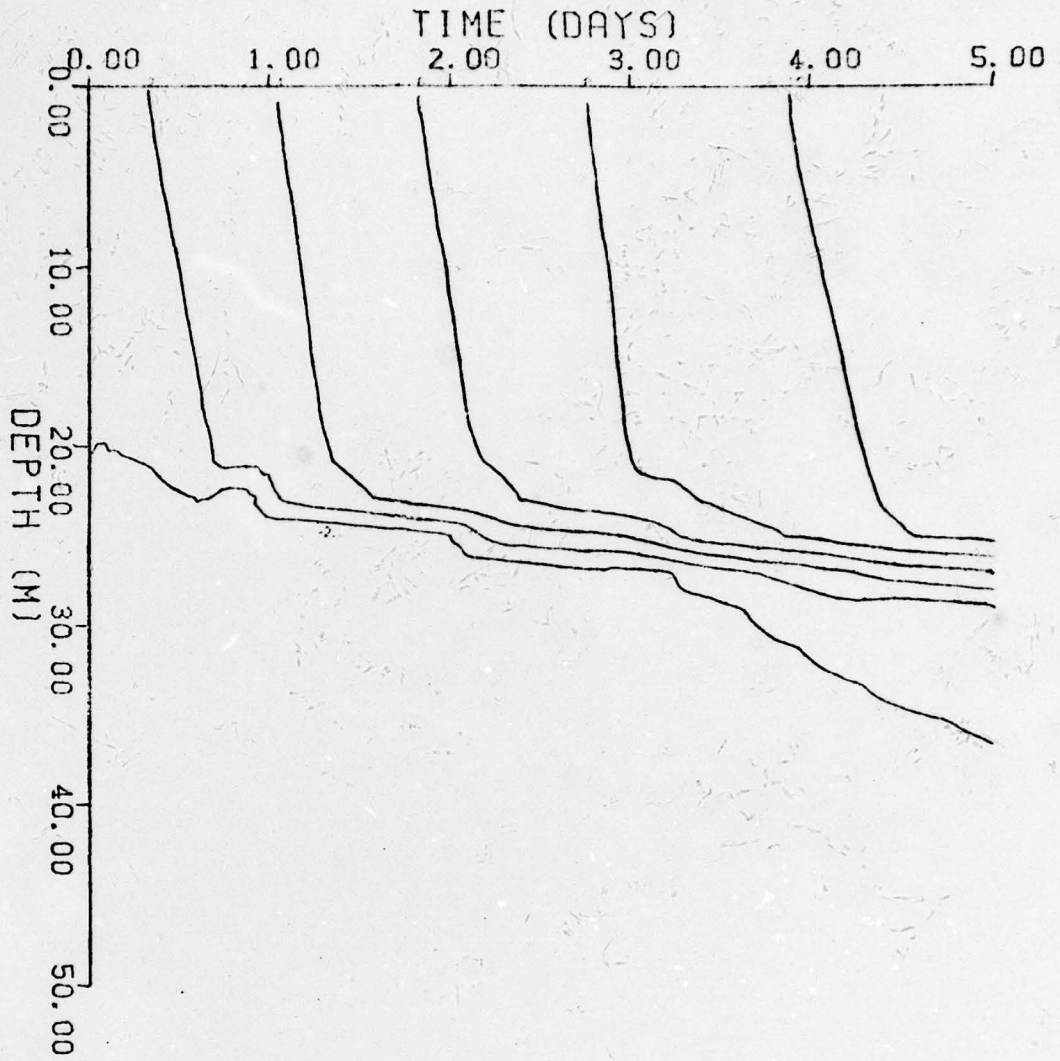
Figure 6. Same as Figure 1 but for Experiment 6 ( \Delta\theta_m = 0 , \Delta q_m = 1 \text{ gm kg}^{-1} , \Delta U_m = 0 , \Delta C = 0 ).
