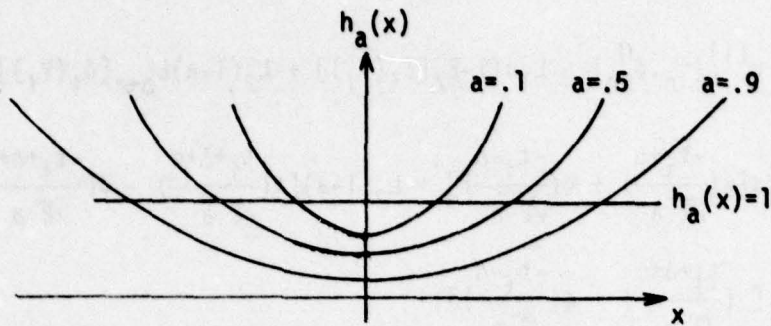
Figure 3. Graph of h_a(x) for a = .1, .5 and .9 .
