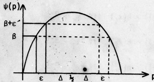
Figure 2. Graph of \psi(p) .
