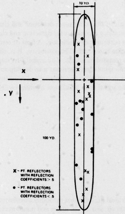
Figure 1. Two dimensional acoustic target model. (U)
