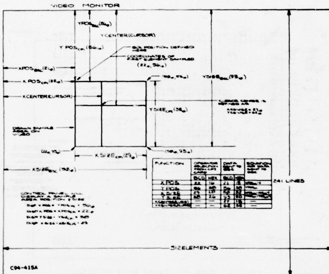
Fig.14. Drawn Sample Area plus Cursor with Term Definitions.
