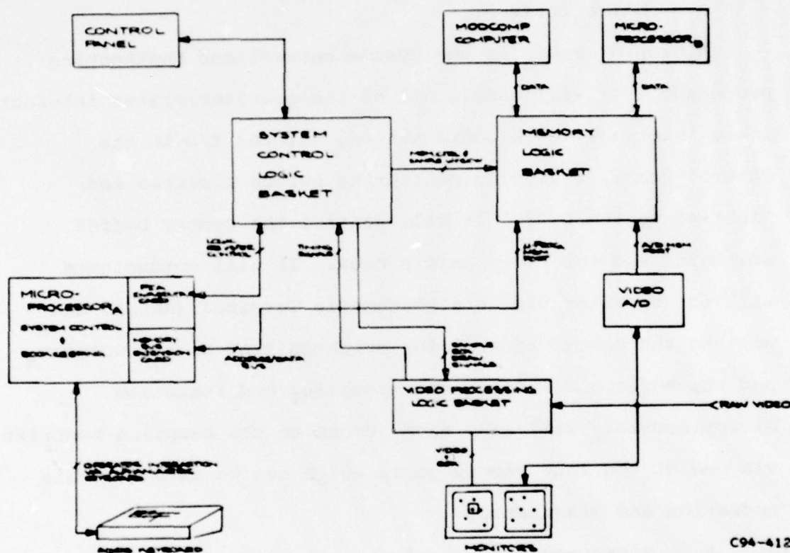
Fig.2. PVDS Hardware Block Diagram.
