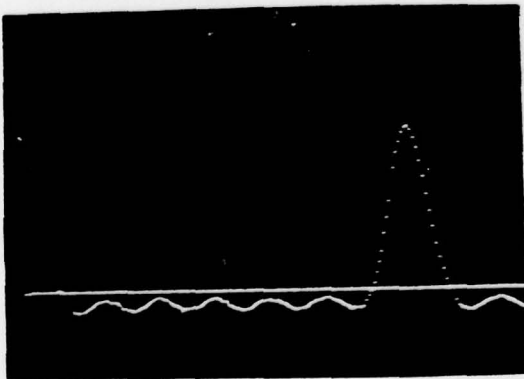
(c) Raised triangular shape; peak is +0.72 V, minimum is -125 mV.
