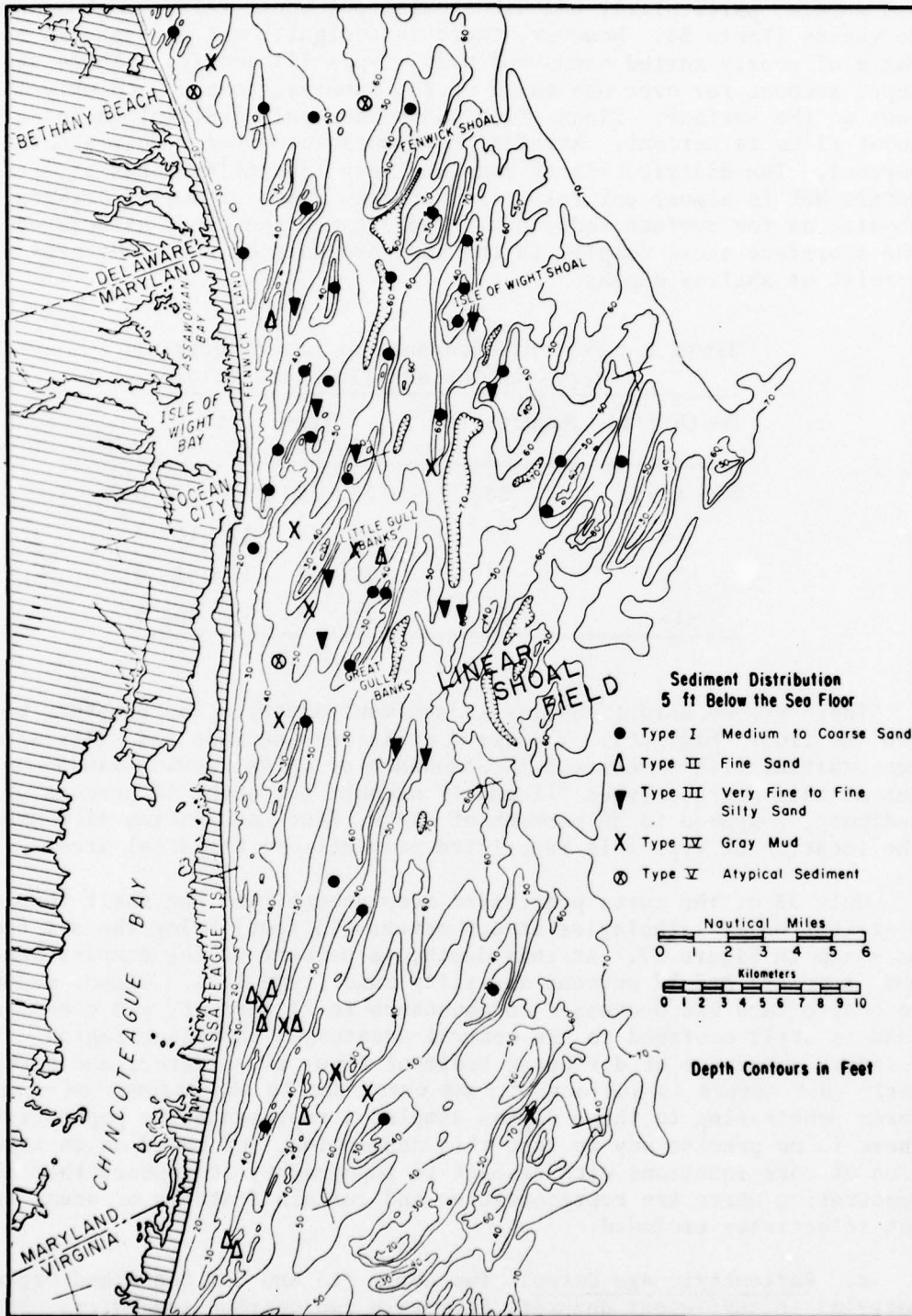
Figure 25. Map showing distribution of major sediment types 5 feet (1.5 meters) below the sea floor in relation to surface topography. Note the close association of type I sands (dots) with shoal areas.
