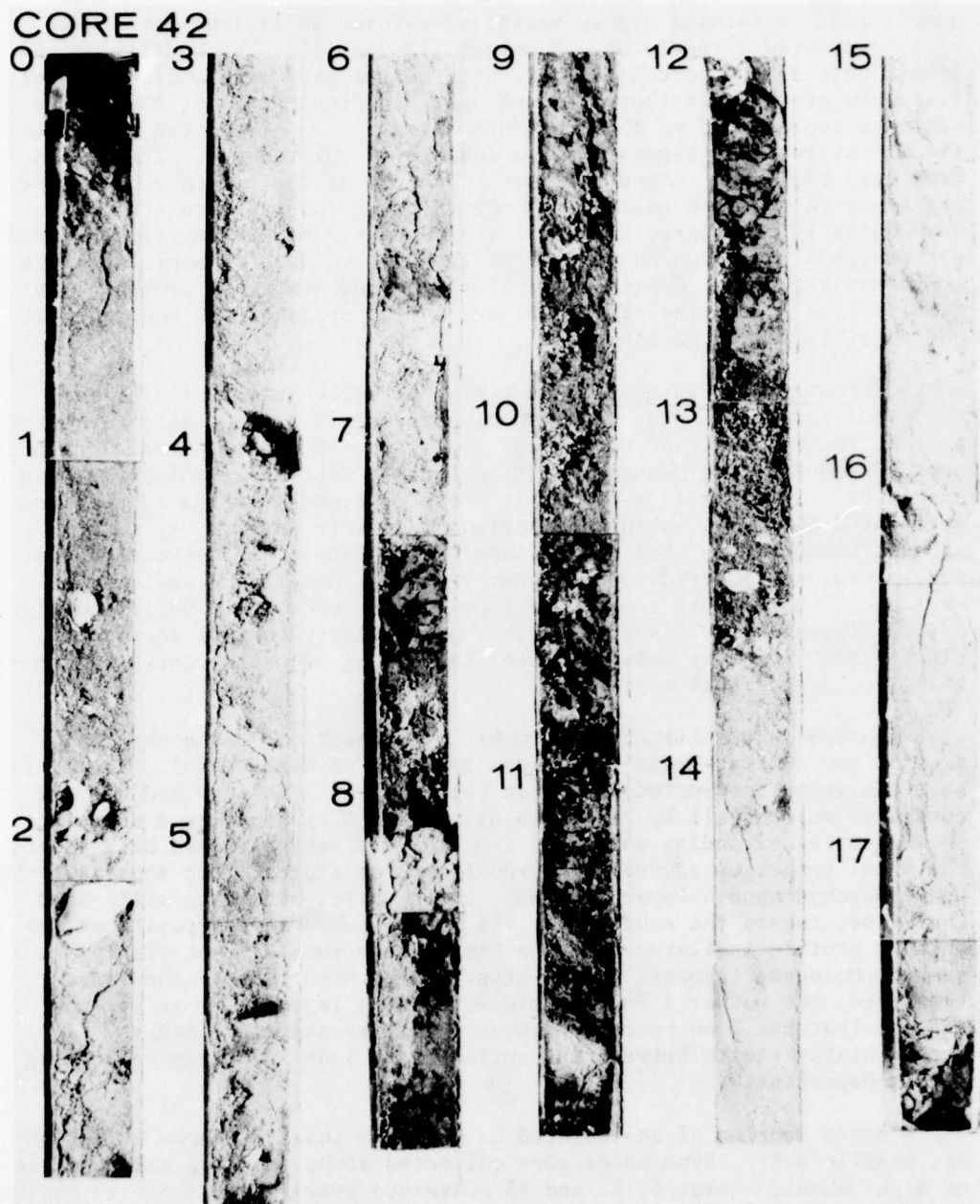
Figure 30. Composite photo of core 42, with sediment depths shown in feet. Lithologic boundaries occur at 2.0, 7.3, 12.9, and 13.7 feet (0.6, 2.2, 3.9, and 4.2 meters). Note whole polycopd values at 1.4 and 2.2 feet (0.43 and 0.67 meter).
