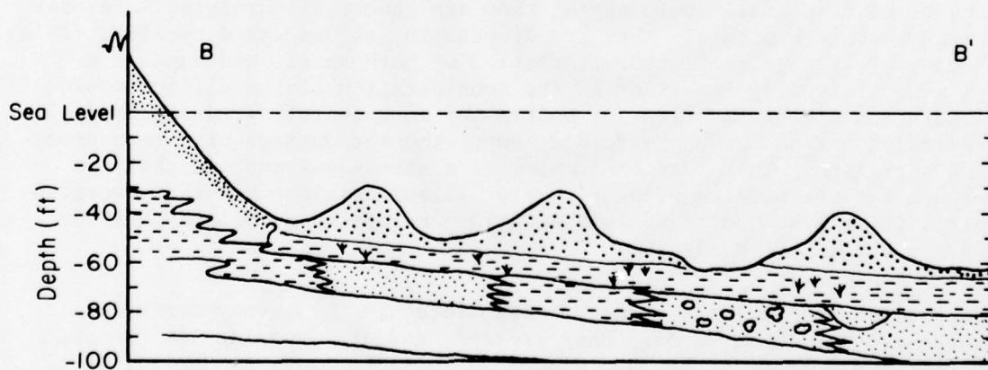
Figure 34. Plan view and representative cross-section profile of the Maryland inner shelf, constructed from seismic and sediment core data. Sediment units correspond to those designated in Figure 33.
