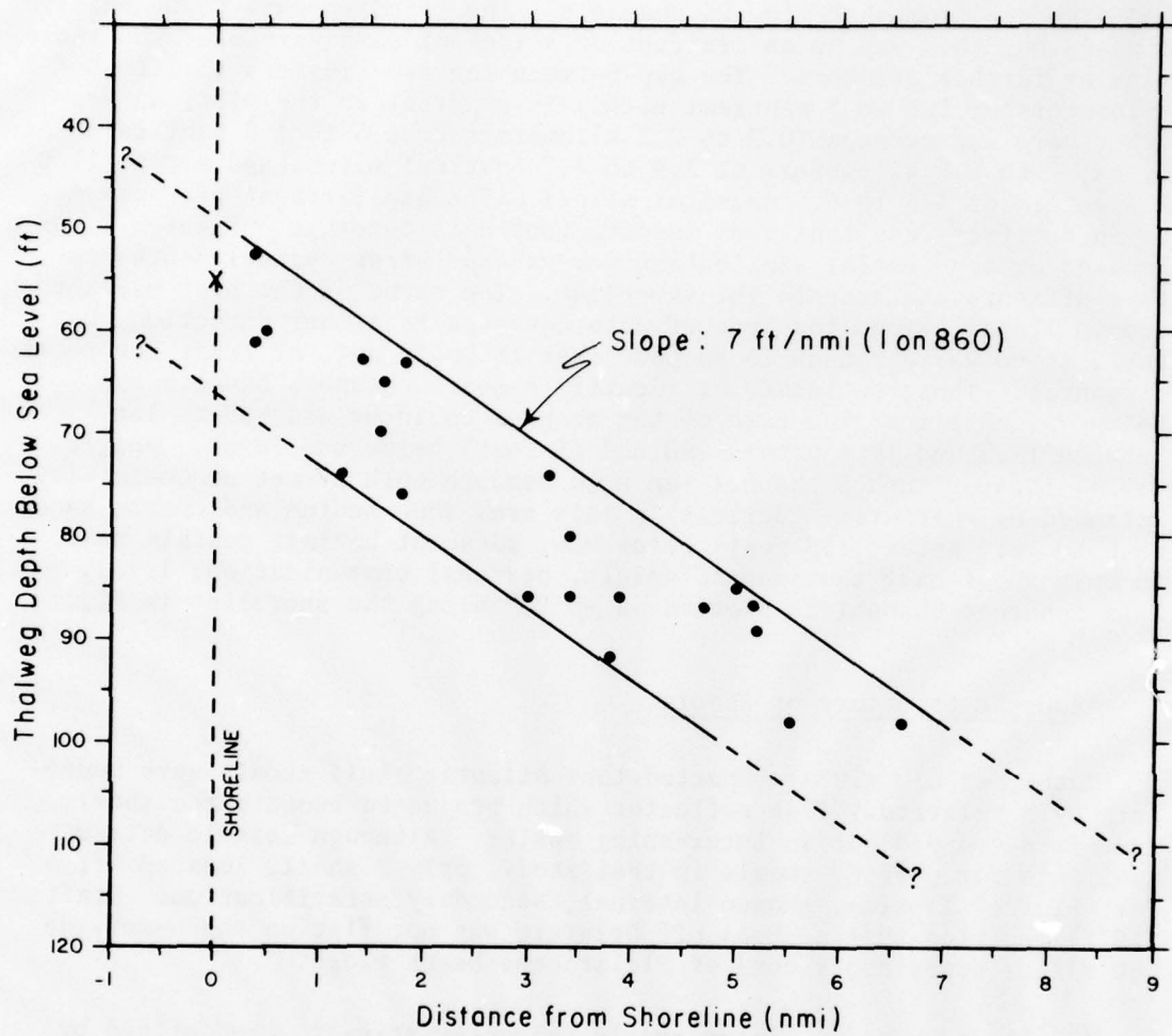
Figure 21. Plot of maximum thalweg depth of buried channels versus distance from shoreline. The X plotted along the shoreline represents sandfilled channel under Ocean City at 66th Street (Weigle, 1974).
