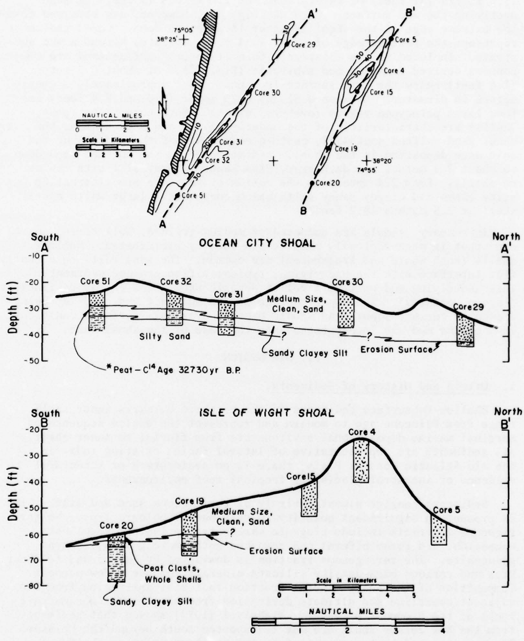
Figure 31. Geologic cross sections along the axes of Isle of Wight and Ocean City shoals. Correlations are based on lithologic comparisons.
