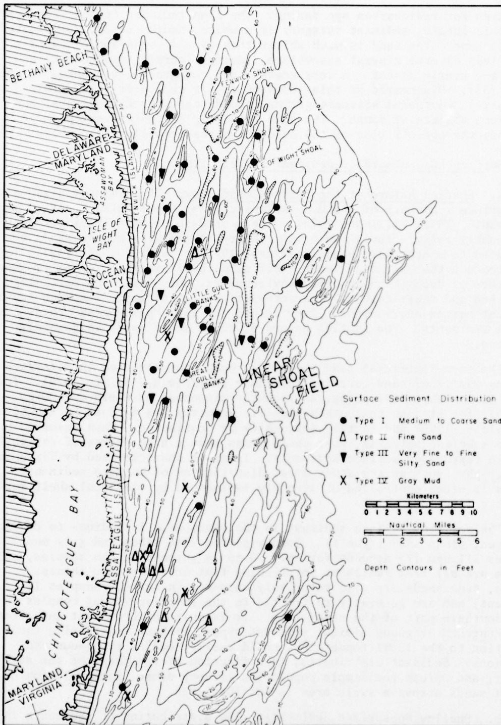
Figure 24. Map showing surface distribution of major sediment types defined in this study in relation to sea floor topography.
