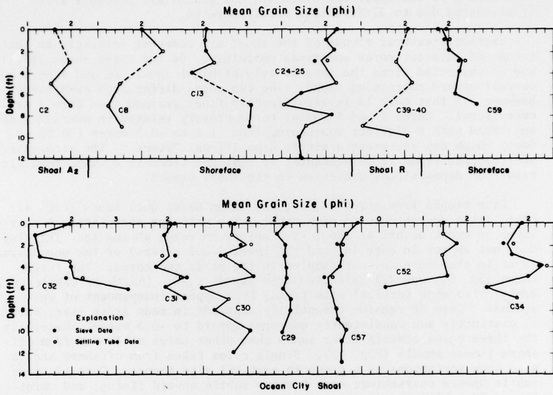
Figure 42. Mean grain size versus depth below sea floor for selected cores collected from the shoreface and shoreface shoals. Data points separated by intervals of 3 feet (1 meter) or more are connected by dotted lines. Settling tube data were corrected to sieve equivalents using an empirically derived formula (see App. B).
