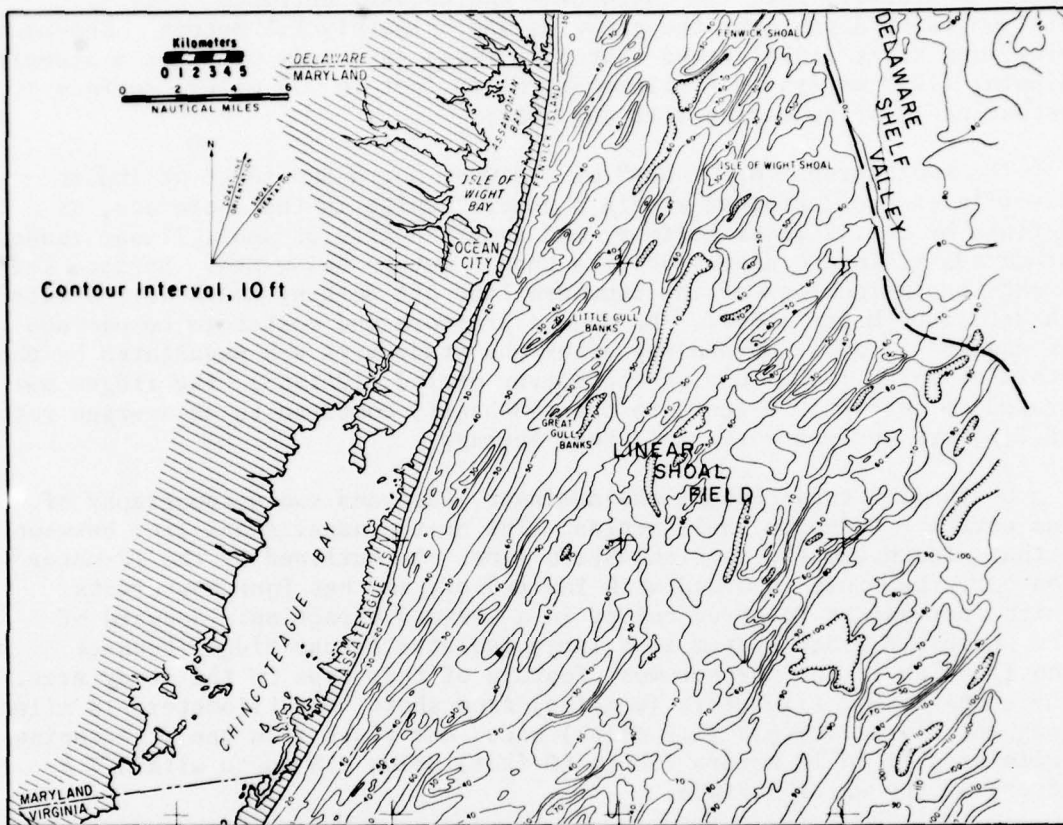
Figure 9. Detailed bathymetry of the Maryland Inner Continental Shelf. Contours compiled from data on NOS chart 1220, scale 1:80,000. Dashline is the approximate boundary between Delaware shelf valley and linear-shoal field.
