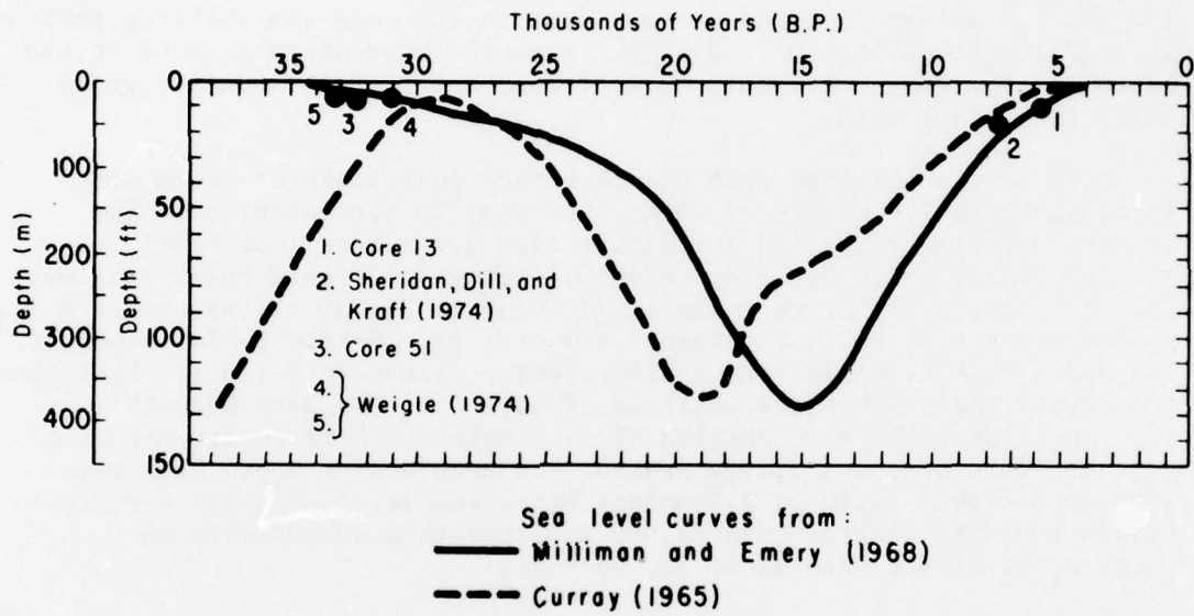
Figure 28. Depth and radiocarbon age of peaty sediments from the study area plotted against two published sea level curves.
