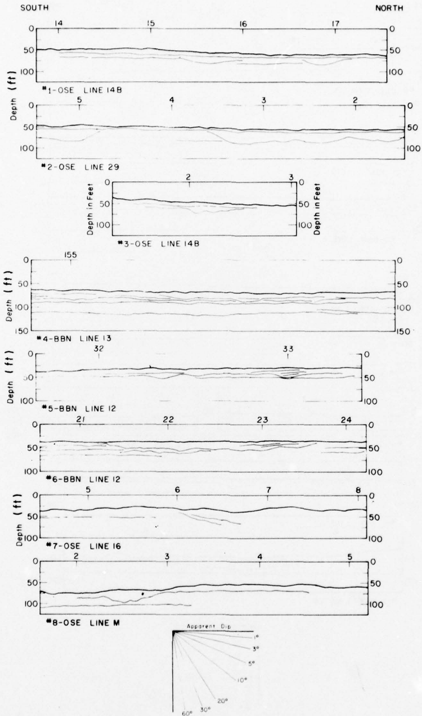
Figure 19. Interpreted acoustic profiles across buried channels on the inner shelf between Bethany Beach, Delaware, and Ocean City, Maryland. A key is provided beneath each profile. The number refers to location in Figure 18; BBN and OSE refer to the Bolt, Beranek and Newman Acoustipulse and Ocean Science and Engineering 3.5-kilohertz transducer; and the line number refers to the tracklines in Figures 2, 3, and 4.
