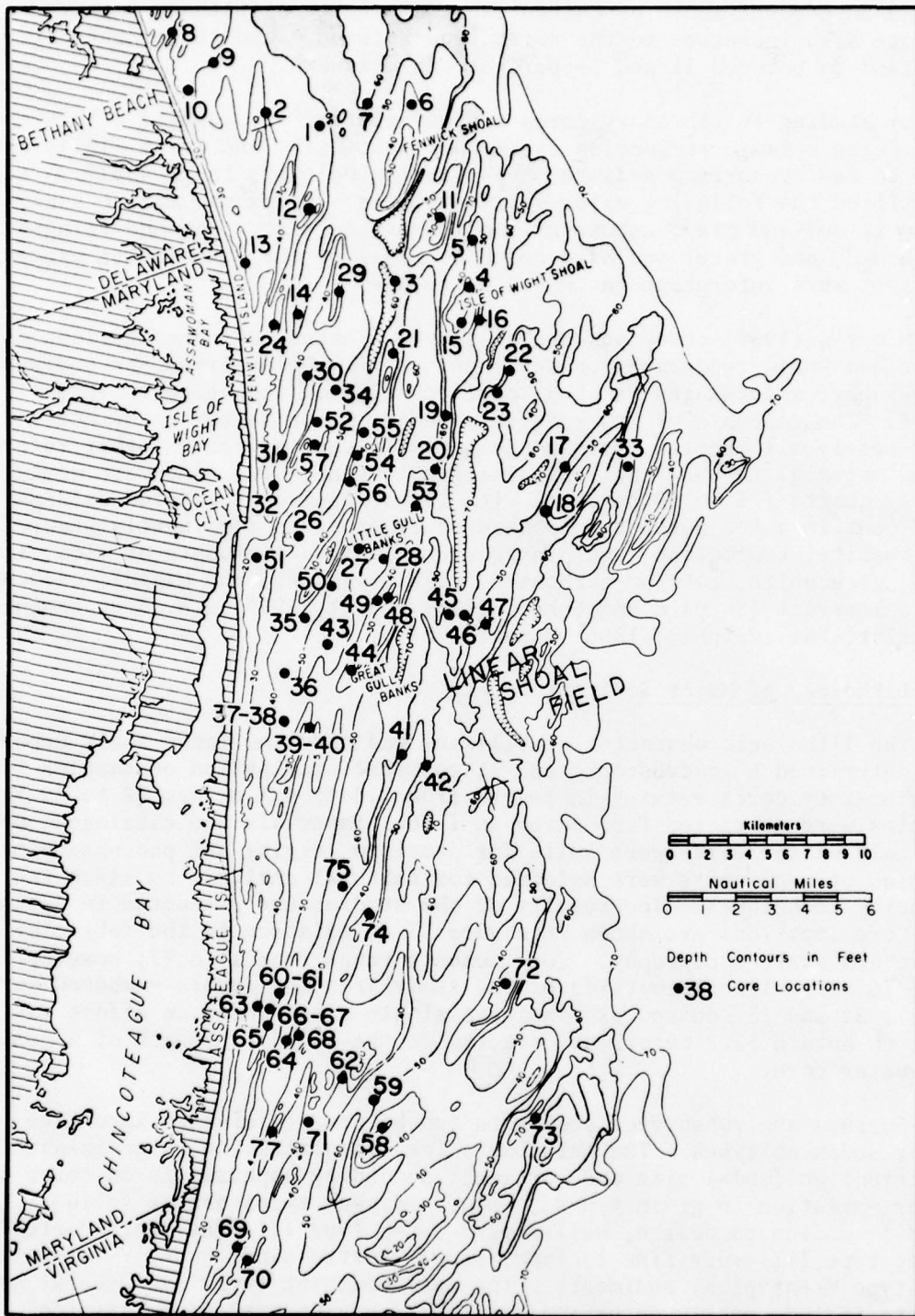
Figure 23. Locations of vibratory cores used in this study shown in relation to shelf topography. Double number (e.g., 37-38) indicates site where attempt was made to obtain one extra long core.
