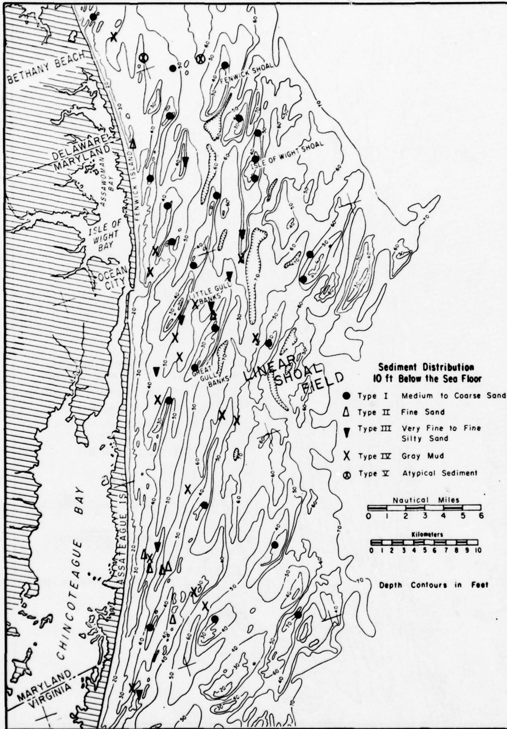
Figure 26. Map showing distribution of major sediment types 10 feet (3.0 meters) below the sea floor in relation to surface topography. Note the close association of type I sands (dots) with shoal areas and the general increase in abundance of mud (X's).
