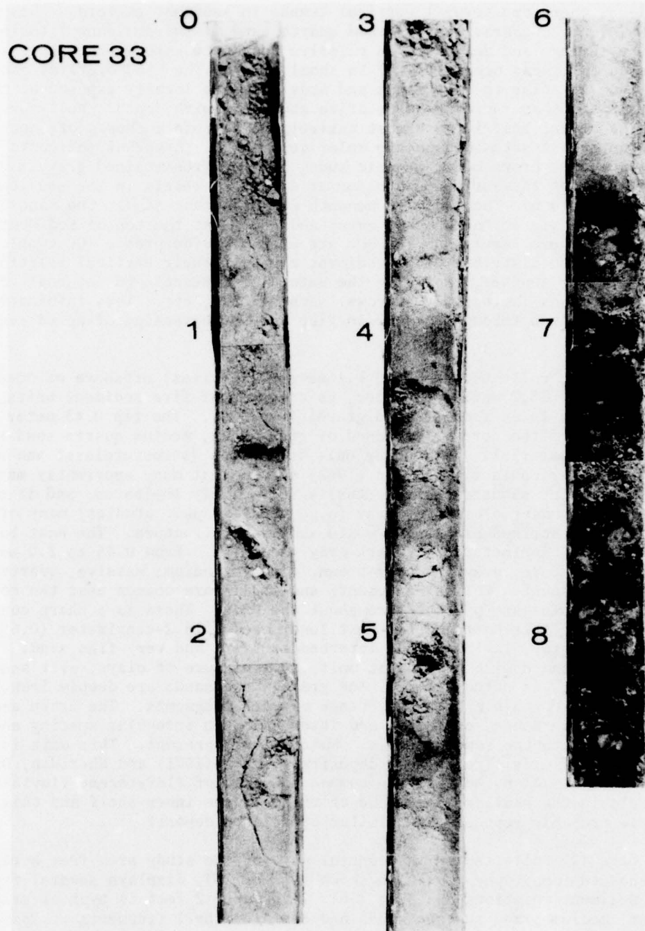
Figure 29. Composite photo of core 33, with sediment depths shown in feet. Lithologic boundaries occur at 1.4, 1.5, 6.6, and 7.2 feet (0.43, 0.46, 2.0, and 2.2 meters). The lowermost unit is a striking red gravel.
