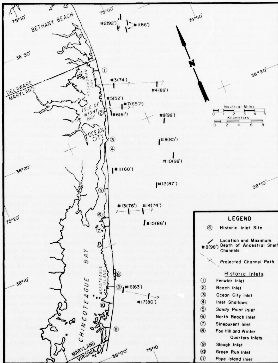
Figure 18. Map showing location and thalweg depths of buried channels on the inner shelf between Bethany Beach, Delaware, and Maryland-Virginia State line. Also shown are locations of historic inlets along the Maryland coast (Truitt, 1967). Channel cross sections are shown in Figures 19 and 20.
