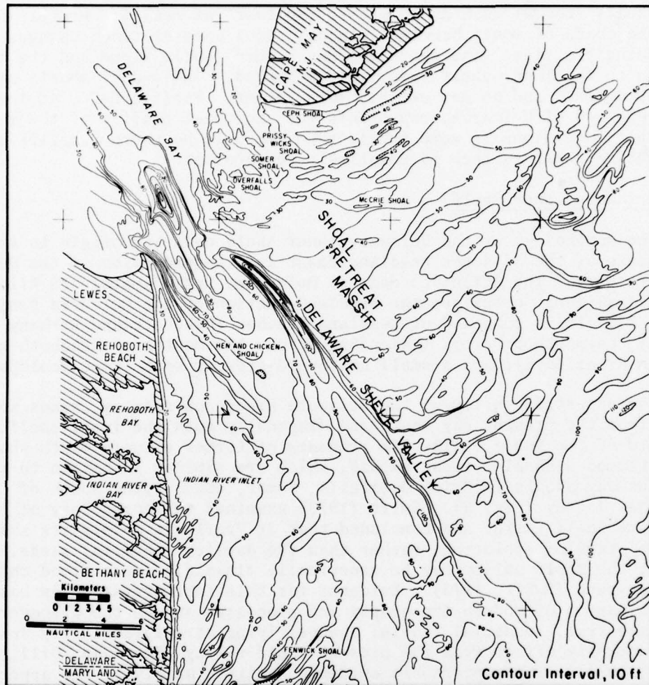
Figure 8. Detailed bathymetry of the Delaware Inner Continental Shelf. Contours compiled from data on National Ocean Survey (NOS) chart 1219, scale 1:80,000.
