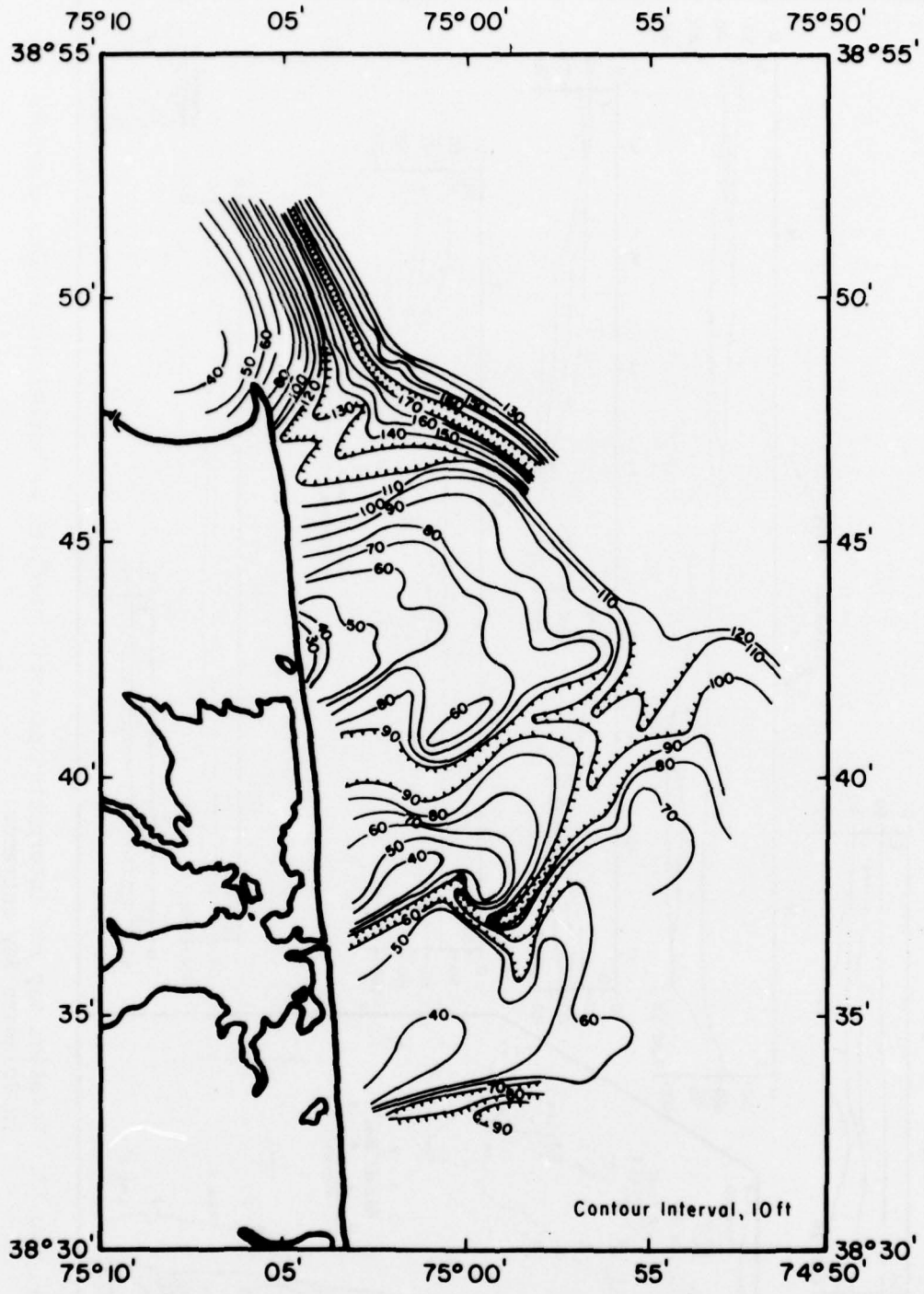
Figure 16. Structure contour map of the pre-Holocene erosional drainage surface off Delaware, modified after Sheridan, Dill, and Kraft (1974).
