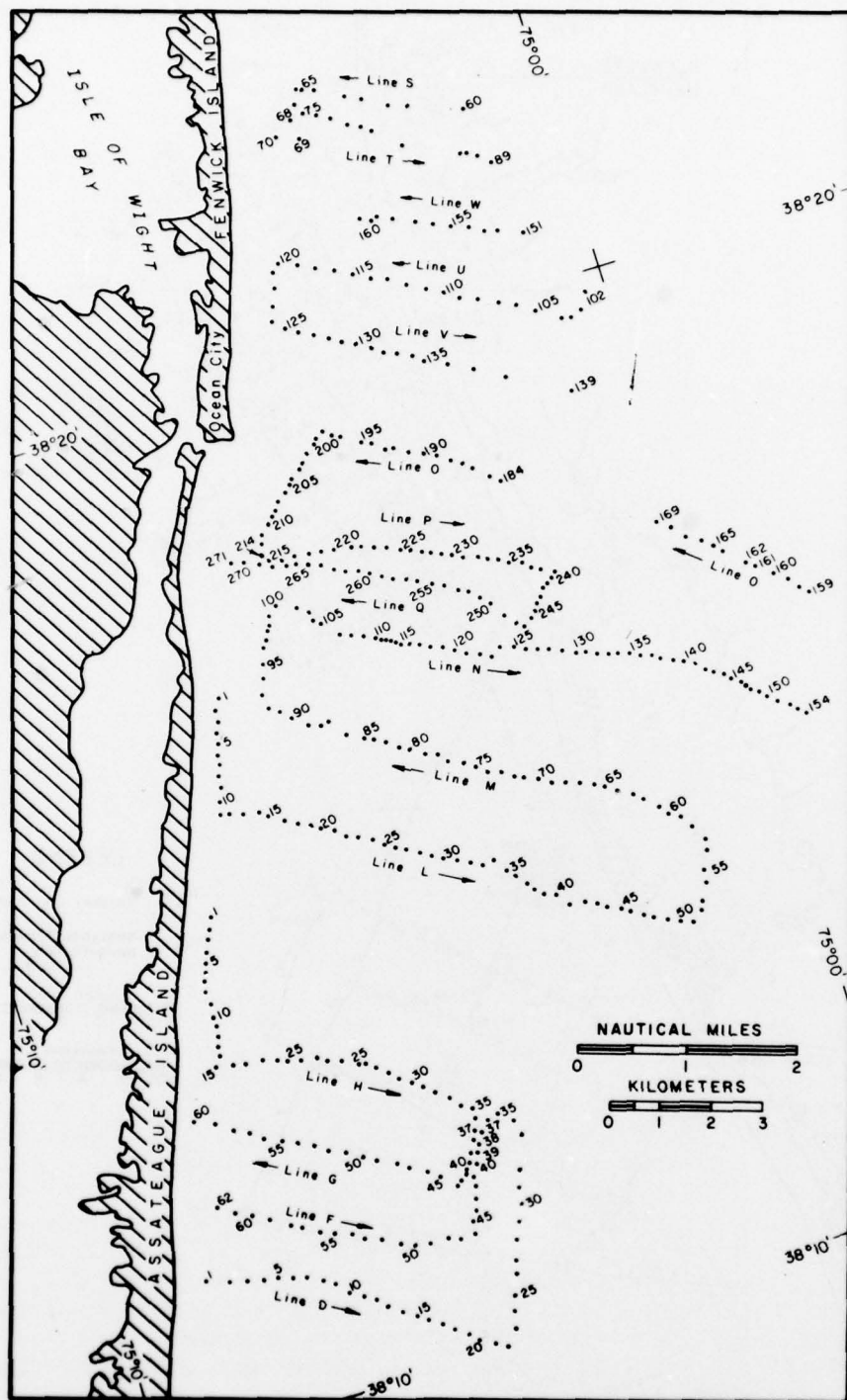
Figure 4. Seismic reflection, fathometer, and side-scan sonar tracklines for linear shoals in the Maryland inner shelf; field data collected spring 1974.
