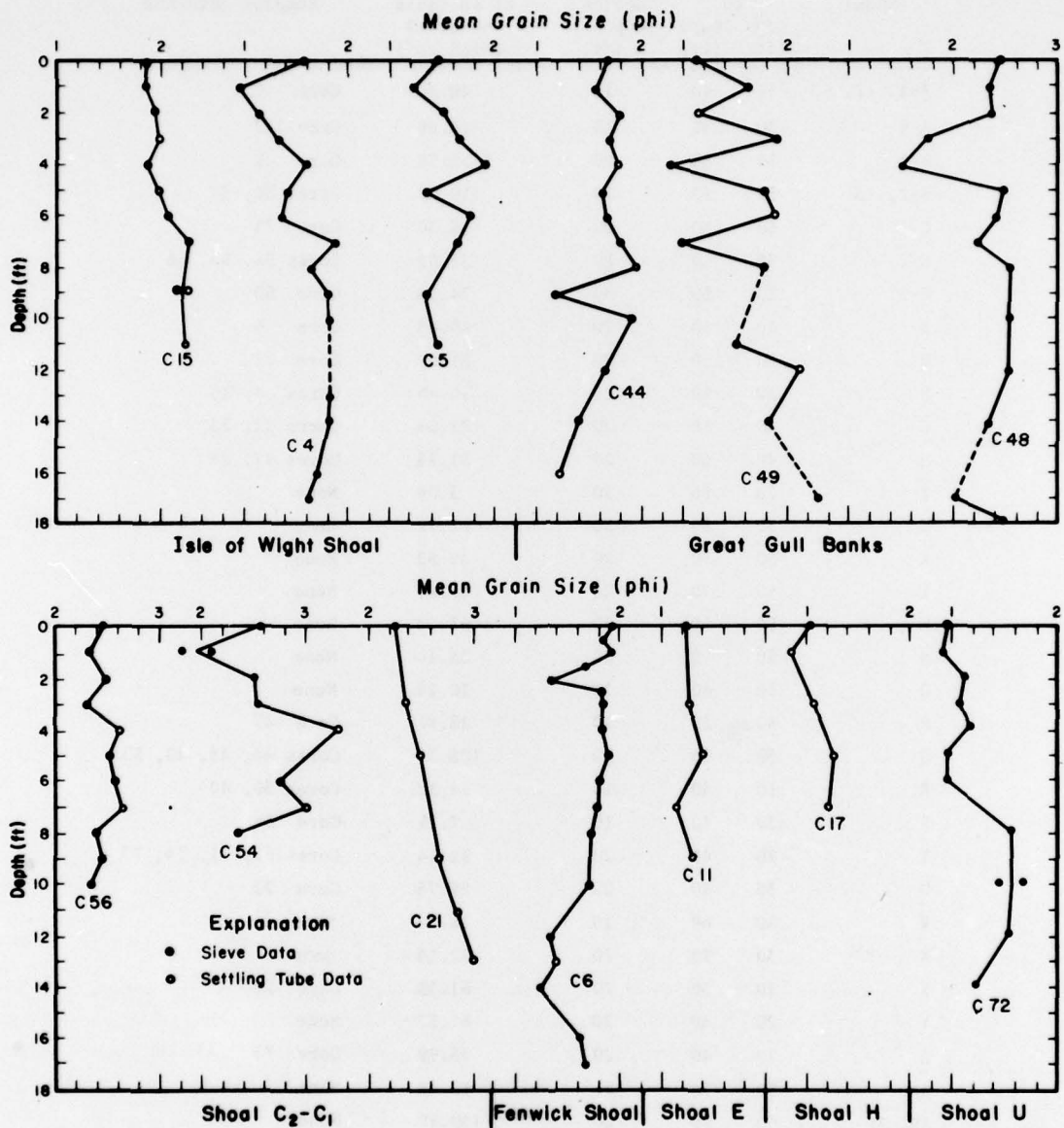
Figure 41. Mean grain size versus depth below sea floor for selected cores from offshore linear shoals. Data points separated by intervals of 3 feet (1 meter) or more are connected by dotted lines. Settling tube data were corrected to sieve equivalents using an empirically derived formula (see App. B).
