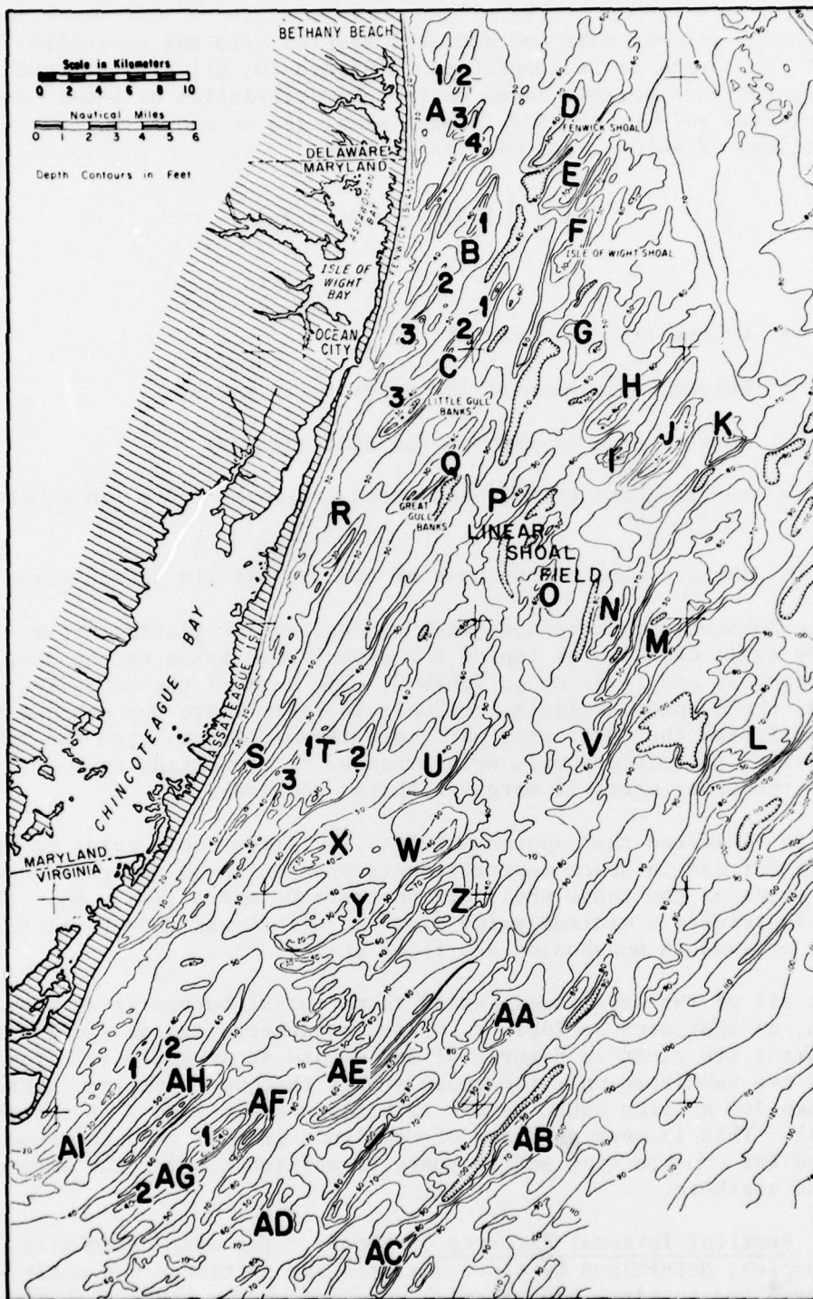
Figure 40. Base map of the shoal field of the northern Delmarva inner shelf indicating potential borrow sites (designated by letter). Borrow sites (shoals) with more than one ridge have numerical subscripts. Contours are compiled from charted depths on NOS chart 1220, scale 1:80,000. Shaded areas are depths shallower than 40 feet (12.2 meters).
