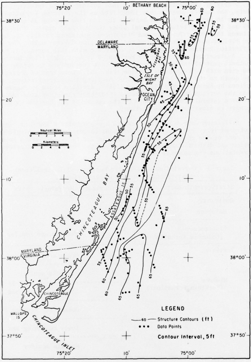
Figure 14. Structure contour map on the surface of the acoustic reflector A 2 . Data points taken from 3.5-kilohertz seismic profile records.
