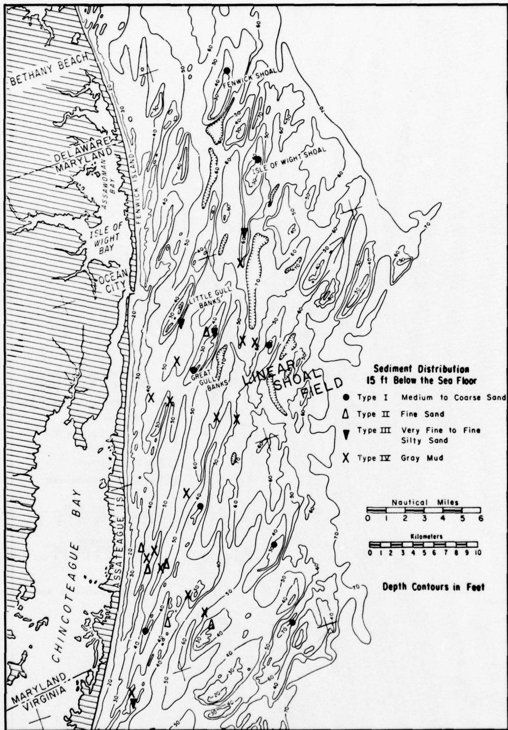
Figure 27. Map showing distribution of major sediment types 15 feet (4.5 meters) below the sea floor in relation to surface topography. Note the close association of type I sands (dots) with shoal areas and the general increase in abundance of mud (X's).
