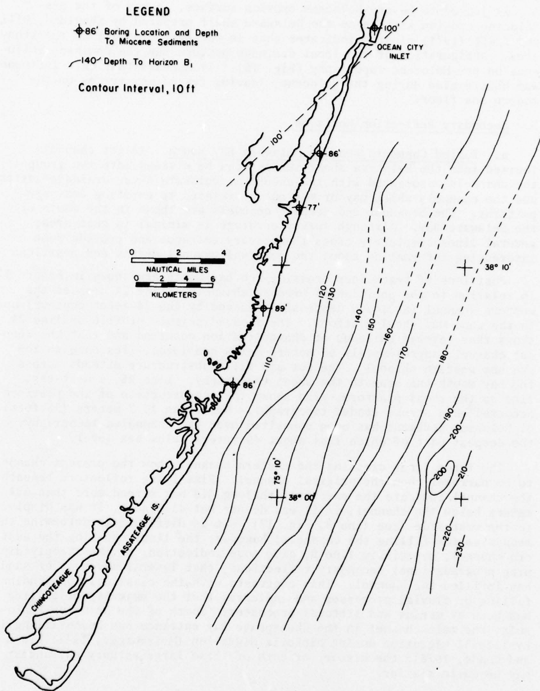
Figure 15. Structure contour map on the surface of acoustic reflector B 1 , the presumed top of the Miocene section. Dashed lines were interpolated. Onshore boring data and contour lines are from Rasmussen and Slaughter (1955).
