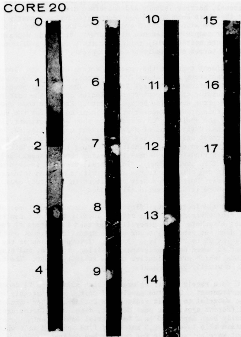
Figure 32. Composite photo of core 20. Location is shown in Figure 31.
