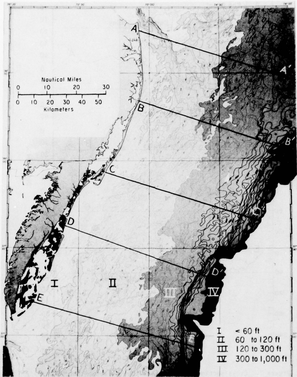
Figure 6. Topography of the Delmarva Continental Shelf showing locations of cross-sectional profiles illustrated in Figure 7.
