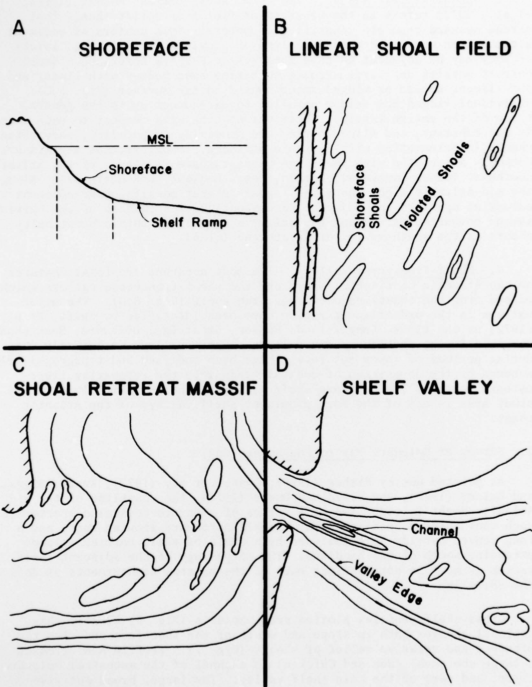
Figure 5. Schematic diagram of four major morphological elements of the northern Delmarva inner shelf.
