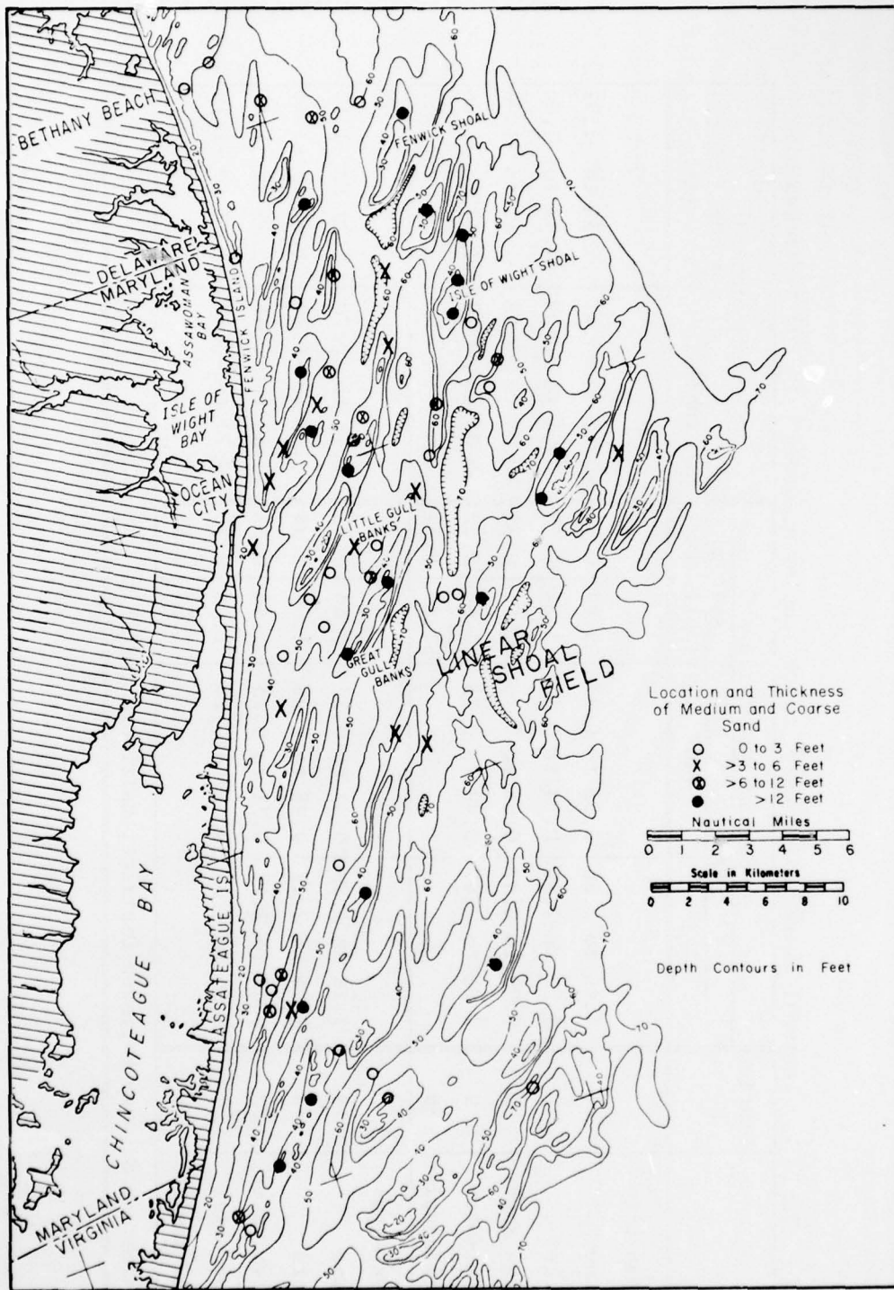
Figure 38. Map showing location and thickness of medium and coarse (modal size) sand in relation to sea floor topography.
