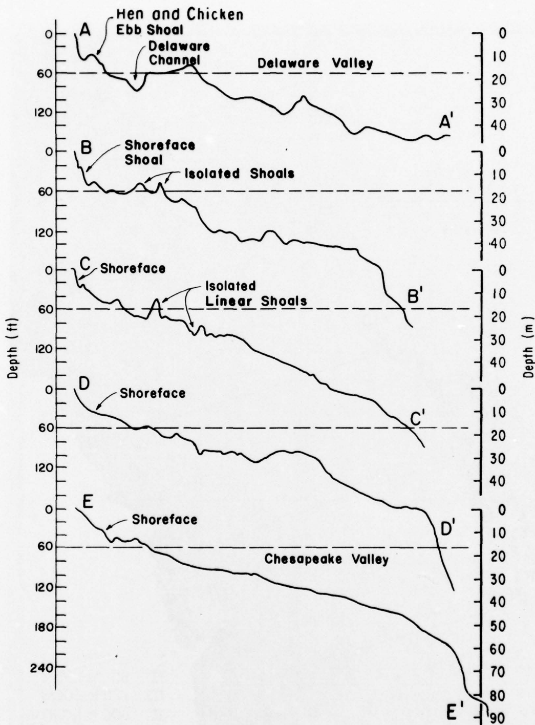
Figure 7. Cross-sectional profiles of the surface of the Delmarva Continental Shelf illustrating major topographic trends. Profile locations are shown in Figure 6.
