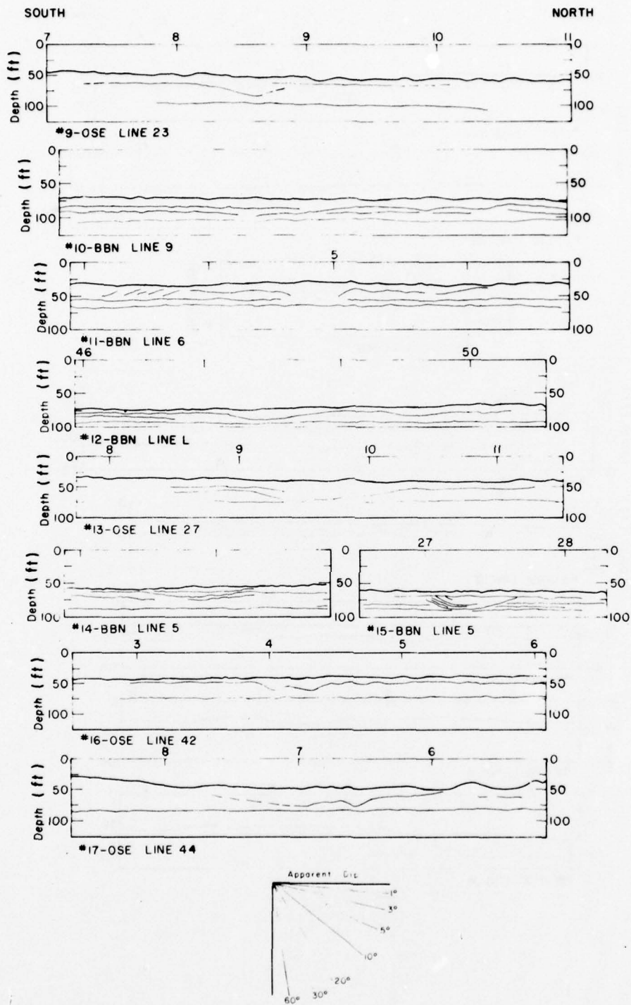
Figure 20. Interpreted acoustic profiles across buried channels on the inner shelf between Ocean City and Virginia State line. A key is provided beneath each profile. The number refers to location in Figure 18; BBN and OSE refer to Bolt, Beranek and Newman Acoustipulse and Ocean Science and Engineering 3.5-kilohertz transducer; and the line number refers to the tracklines in Figures 2, 3, and 4.
