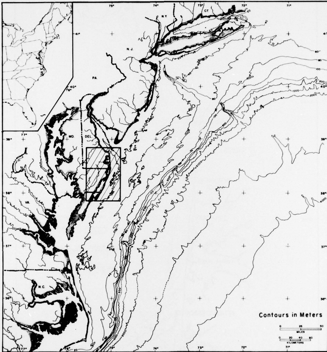
Figure 1. Regional setting of the study area. The inner shelf of Delaware, Maryland, and northern Virginia is centered in the U.S. mid-Atlantic geologic province.
