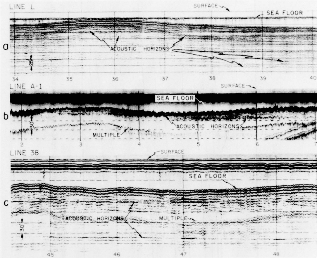
Figure 12. Acoustic records produced by the three types of seismic reflection equipment used in this study--(a) Acoustipulse (multiple transducers) record, (b) 3.5-kilohertz (single transducer) record, and (c) engineering sparker records.
