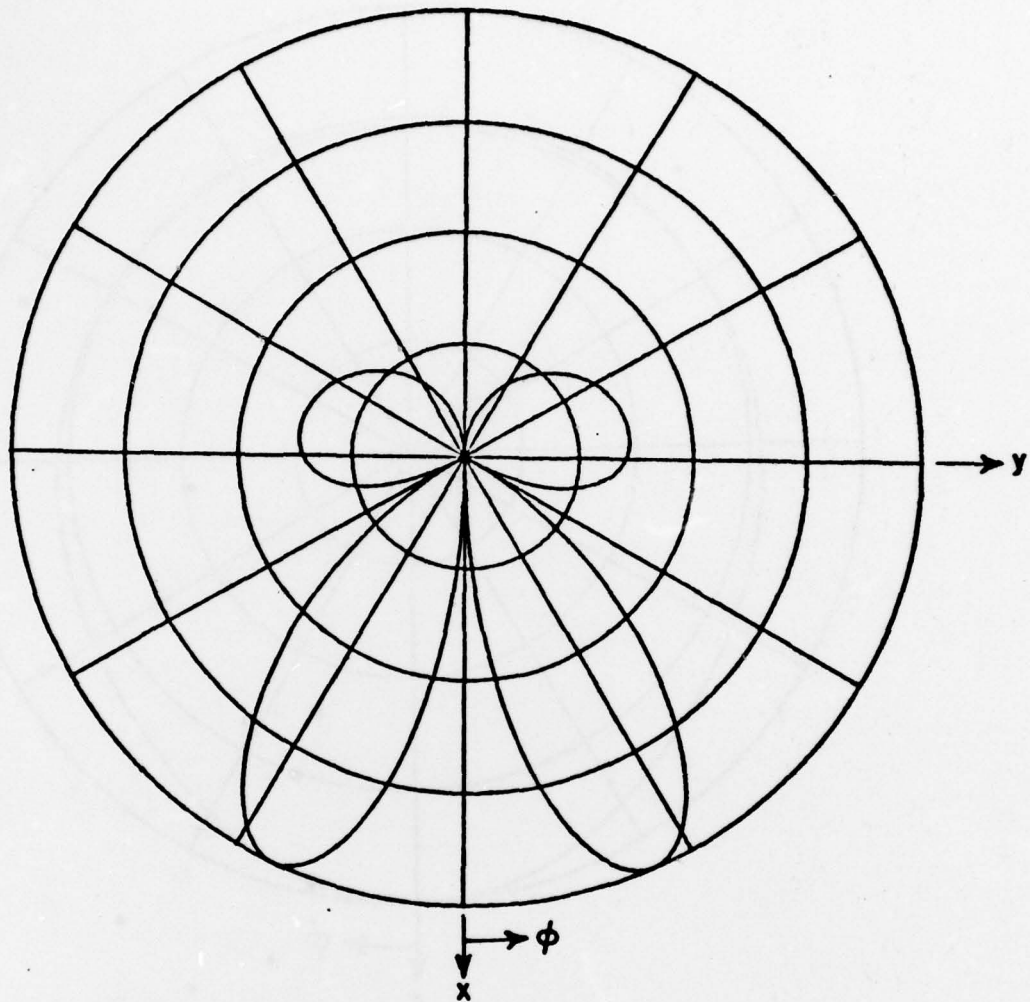
Figure 73. H_z field distribution of R-line of Figure 66 in free space around a concentric circle of radius r=1 meter. f=100 MHz. Goubau-like mode.
