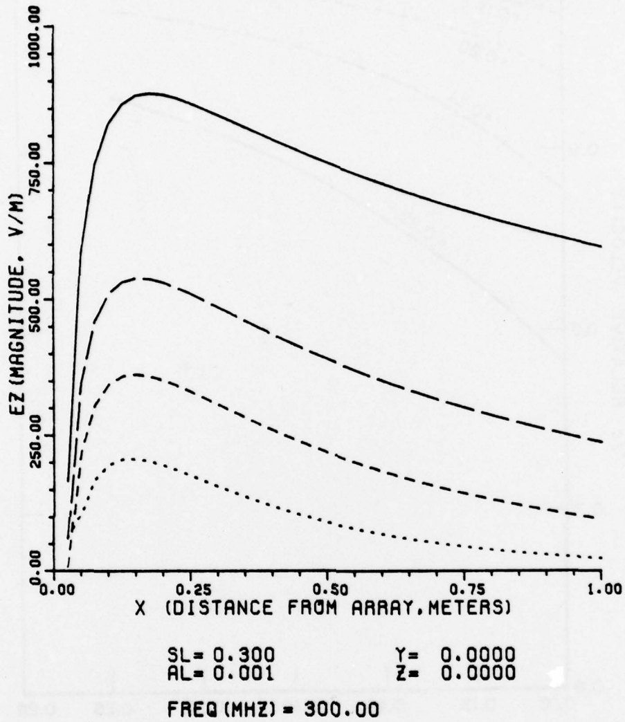
Figure 13. z-component of E-field in a transverse cut in plane of a dipole, normalized such that current at center of each dipole is 1 Amp. a/\lambda=0.001 , s/\lambda=0.30 , f=300 MHz.
