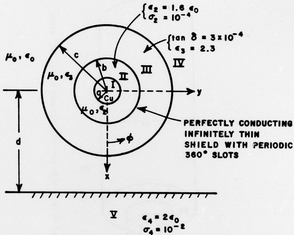
Figure 60. Cross-section of an infinitely long coaxial cable with periodic circumferential 360° slots over a flat earth.
