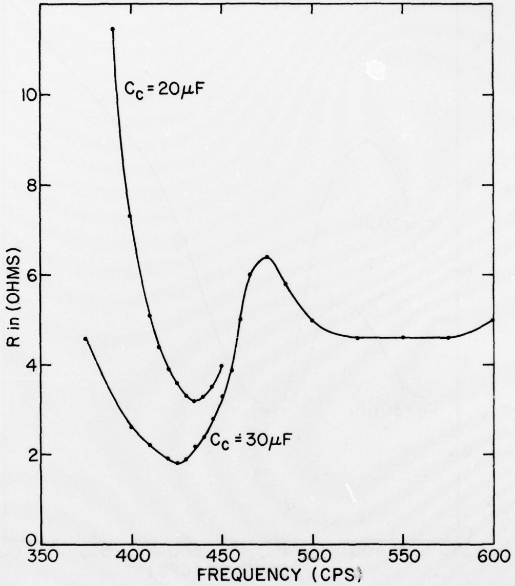
Figure 10 - Input resistance
