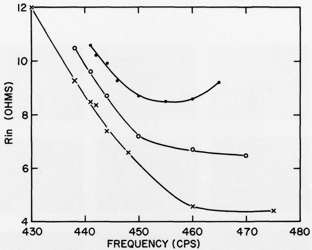
Figure 16 - Input resistance
