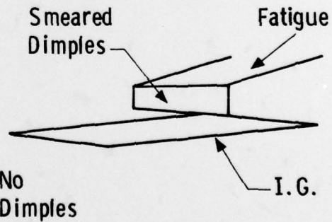
Fig. 8.11 -Cracking sequence in H 2 test leading to a fracture appearance a) similar to that of Fig.8.10 (iv) and b) a featureless zone overhanging an intergranular fracture as found in Fig. 8.6
