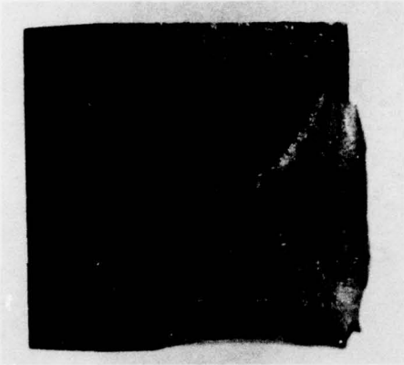
Figure 4-9 - Weld-metal Charpy specimen QS1-1 fracture, showing diagonal H 2 S crack front
