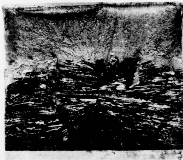
Fig. 3-5 Optical macrograph of fracture surface of Specimen P-C. A scanning electron microscope view of the intergranular fracture surface is shown in Fig. 3-8.
