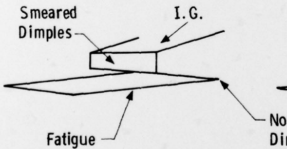
Fig. 8.11 -Cracking sequence in H 2 test leading to a fracture appearance a) similar to that of Fig.8.10 (iv) and b) a featureless zone overhanging an intergranular fracture as found in Fig. 8.6
