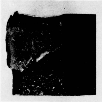
Figure 4-6 - HY-130 weld metal Charpy specimen F1-3 fracture showing arc-shaped H 2 S crack front in only lower (coarse-grained) half of specimen
