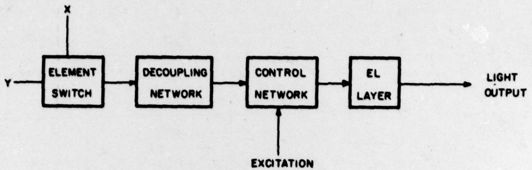
FIGURE 1 - Block Diagram of Single Electroluminescent Element
