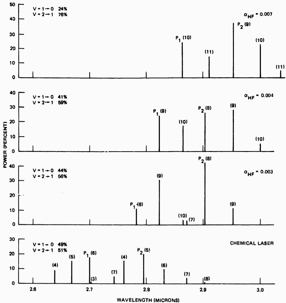
Figure 23. Multiple cell output spectra (76 torr, 0.65 \times 10^3 cm/sec).
