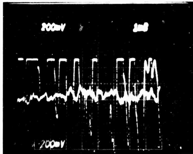
Figure 29. Extracavity ORTL temporal characteristics near threshold.
