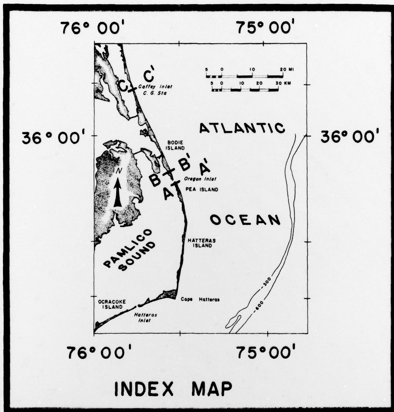
Fig. 10. Location of profiles and shallow borings, Outer Banks, North Carolina.
