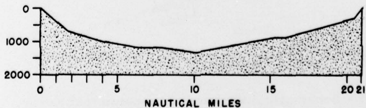
Fig. 2 - Saddleback Cay - Goulding Cay cross section
