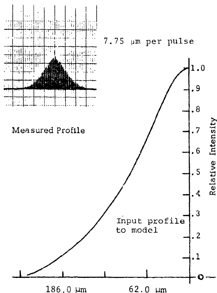
Figure 7. Measured and model relative-intensity profile for dye cell. (\lambda = 514.5 \text{ nm}; 1/e^2 \text{ power radius} = 172.5 \text{ } \mu\text{m}) .
