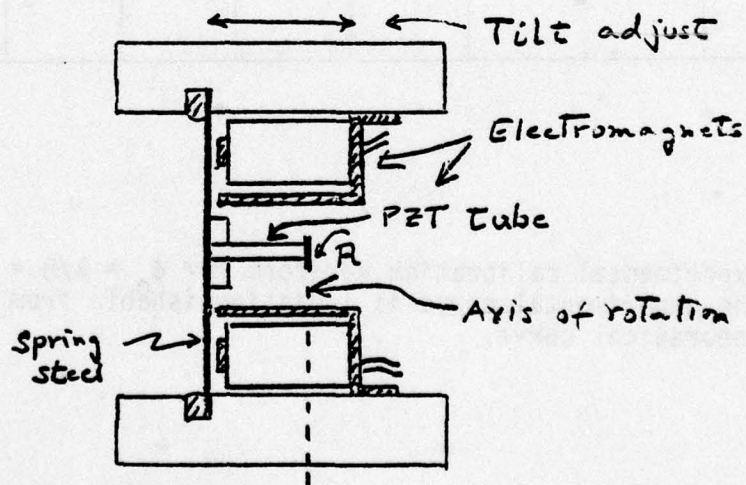
Figure II-6. Optical path correction unit. The PZT tube corrects for \sim 6 fringes with response time \sim 1 msec; the electromagnets correct for \sim 6000 fringes with response time \sim 100 msec.
