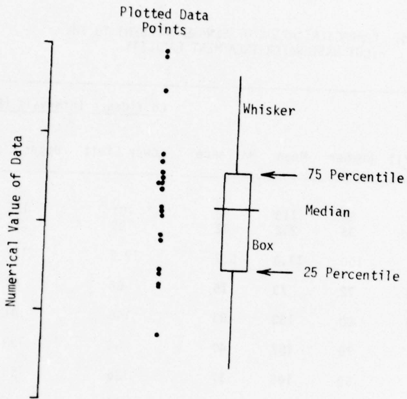
Figure 5. Box-and-Whisker Illustration.
